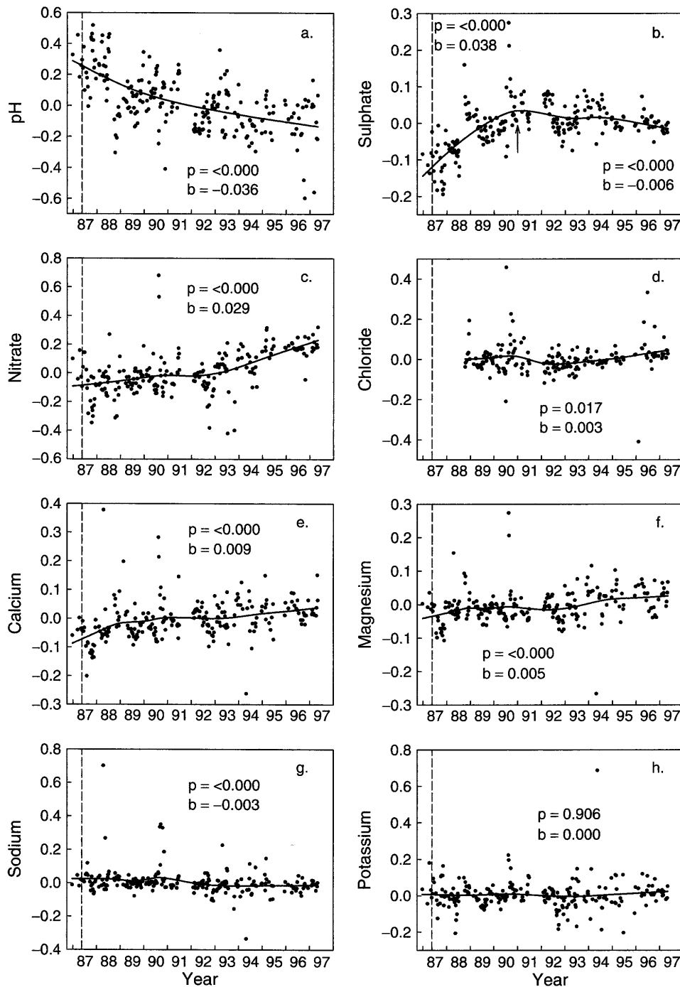
Figure 6. Residuals representing log-transformed baseflow concentration changes over time on WS9 as a result only of the acidification treatment: (a) pH; (b) \text{SO}_4 ; (c) \text{NO}_3 ; (d) Cl; (e) Ca; (f) Mg; (g) Na; (h) K. Trend lines were developed using robust locally weighted regression. The p -value is the Mann-Kendall probability of a significant monotonic trend over time, and b is the Sen slope estimate of the trend. An arrow indicates where the RLW trend-line changed directions and trend and slope tests were performed on data on either side of the arrow. Treatment began in 1987 (dashed line)
