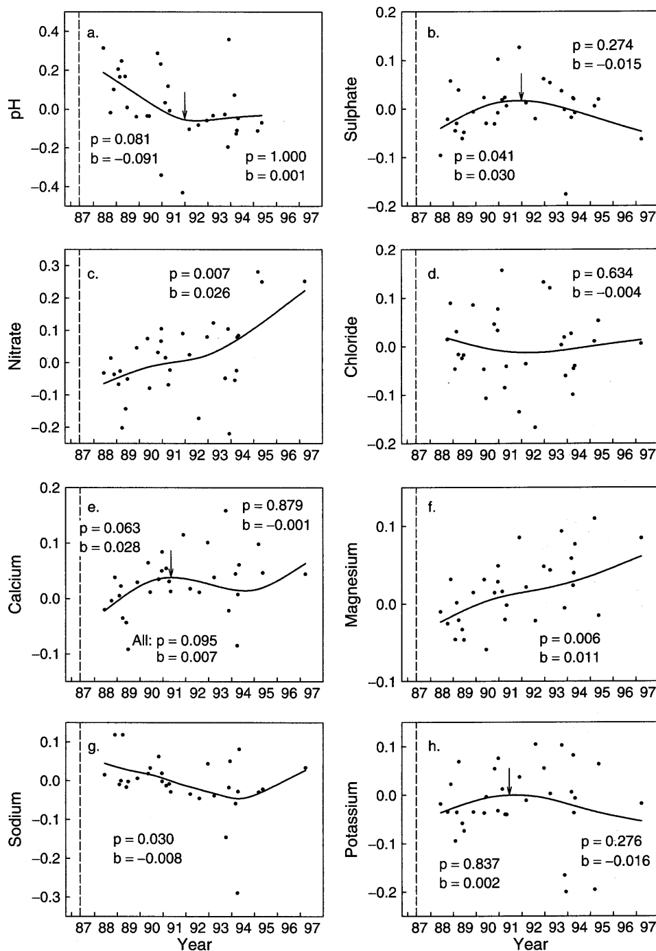
Figure 7. Residuals representing log-transformed peakflow concentration changes over time on WS9 as a result only of the acidification treatment: (a) pH; (b) \text{SO}_4 ; (c) \text{NO}_3 ; (d) Cl; (e) Ca; (f) Mg; (g) Na; (h) K. Trend lines were developed using robust locally weighted regression. The p -value is the Mann-Kendall probability of a significant monotonic trend over time, and b is the Sen slope estimate of the trend. An arrow indicates where the RLW trend-line changed directions and trend and slope tests were performed on data on either side of the arrow. Treatment began in 1987 (dashed line)
