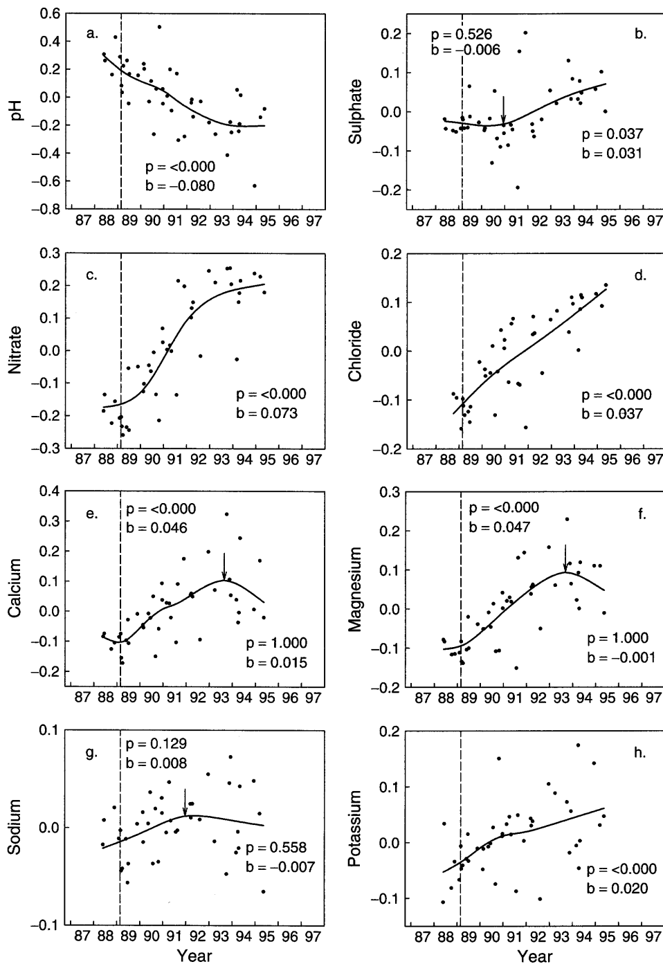
Figure 5. Residuals representing log-transformed peakflow concentration changes over time on WS3 as a result only of the acidification treatment: (a) pH; (b) \text{SO}_4 ; (c) \text{NO}_3 ; (d) Cl; (e) Ca; (f) Mg; (g) Na; (h) K. Trend lines were developed using robust locally weighted regression. The p -value is the Mann–Kendall probability of a significant monotonic trend over time, and b is the Sen slope estimate of the trend. An arrow indicates where the RLW trend-line changed directions and trend and slope tests were performed on data on either side of the arrow. Treatment began in 1989 (dashed line)
