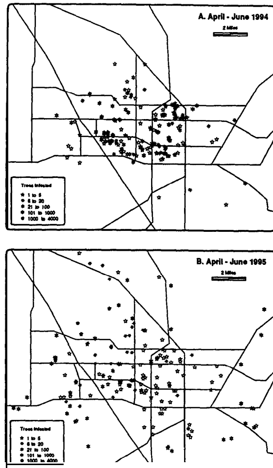
Figure 1. Comparison of SPB infestation size and location during the April-June periods of (a) 1994 and (b) 1995. The rapid detection and destruction of SPB brood clearly reduced the number and severity of infestation in the urban area, but failed to keep infestations from developing over a larger area.
