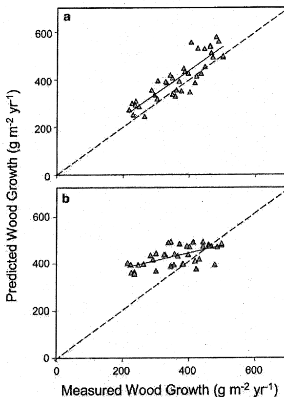
Figure 12. Predicted versus observed wood growth using two alternative methods of obtaining foliar N model input data. In (a), PnET-II was run for individual field plots using species-specific foliar N values from samples collected at each plot ( R^2 = 0.79 , SEE = 39.4 \text{ g m}^{-2} \text{ year}^{-1} ). These results correspond to the 'Measured-N' predictions referred to in the text. In (b) PnET-II was run using mean % N values for deciduous and evergreen species, averaged over all plots at Bartlett ( R^2 = 0.37 ), representing a typical modeling scenario where plot-by-plot foliar N estimates were unavailable. These results correspond to the 'Mean-N' predictions referred to in the text. Dashed lines show the 1:1 relationships.
