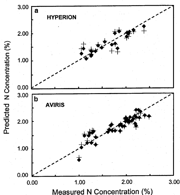
Figure 6. Predicted versus observed canopy nitrogen concentration based on PLS regression models using (a) HYPERION and (b) AVIRIS absorbance data. In both panels diamonds represent the calibration model and crosses represent the validation model. Dashed lines represent the 1:1 relationship.
