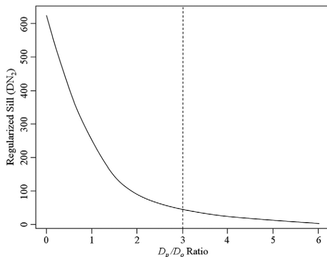
Fig. 3. Negative curvilinear effect of regularization on sill variance as D_p/D_o ratio increases. Sills initially exhibits a steep rate of decrease from punctual variance then become much less sensitive to regularization at D_p/D_o > 3 . The function remains constant despite either pixel ( D_p ) or canopy ( D_o ) size. Adapted from Song and Woodcock (2002).
