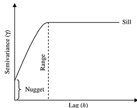
Fig. 2. Classic semivariogram shape for stationary data or imagery. The diagnostic parameters of the semivariogram are the range, sill, and the nugget effect.
