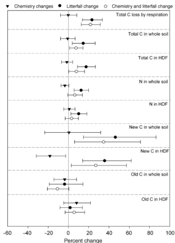
Fig. 6 Percentage changes in soil C and N concentrations in 1.0 g elevated \text{CO}_2 litter (–▼– chemistry change), 1.4 g ambient litter (–●– litterfall change) and 1.4 g elevated \text{CO}_2 litter (–○– chemistry and litterfall changes) compared with 1.0 g ambient litter after incubation for 230 days. Litter and soil were collected from either ambient or elevated \text{CO}_2 treatments at the Aspen FACE experiment, Rhinelander, WI, USA. Results are grouped by parameters. Symbols are means \pm 95% confidence intervals ( n = 5 ). The percentage changes were significantly different from 0 as the confidence interval did not overlap with 0.
