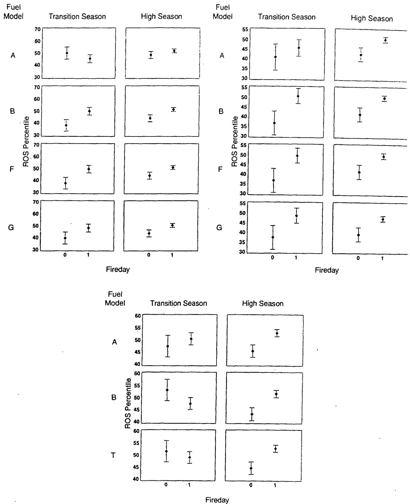
Figure 6. Means and 95.0 percent Tukey HSD intervals for ROS percentile values by Fireday, by NFDRS fuel model, for: (a) the Santa Clara ranger unit; (b) the Nevada-Yuba-Placer ranger unit; and (c) the Riverside ranger unit.
