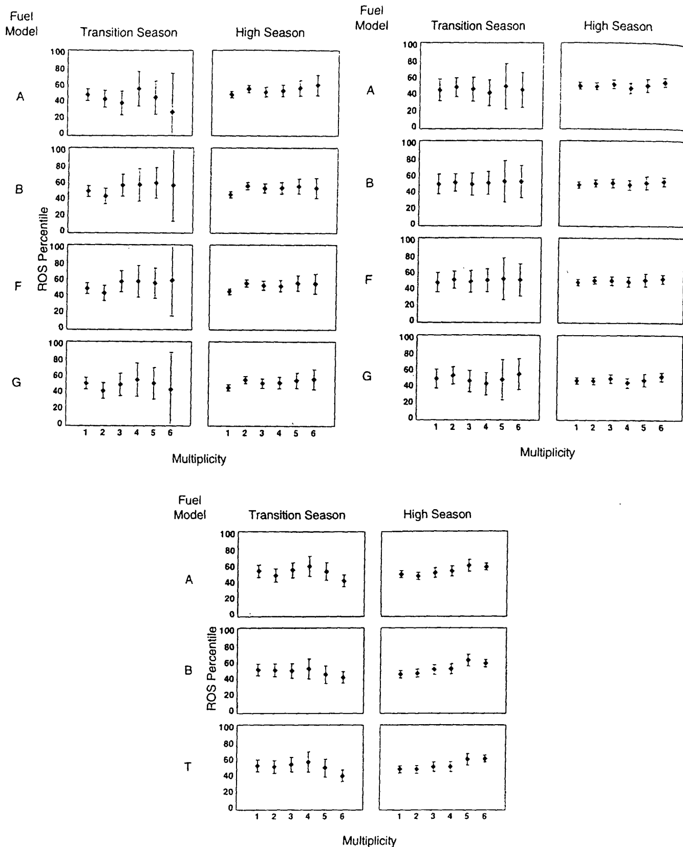
Figure 7. Means and 95.0 percent Tukey HSD intervals for ROS percentile values by Multiplicity, by NFDRS fuel model, for: (a) the Santa Clara ranger unit; (b) the Nevada-Yuba-Placer ranger unit; and (c) the Riverside ranger unit.
