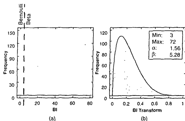
Figure 4. BI, calculated using data from AFFIRMS weather station 43903, fuel model A, slope class 2, high fire season: (a) frequency histogram, with dashed vertical line defining ranges modeled with Bernoulli (left) and beta (right) distributions; (b) beta range frequency histogram and fitted beta distribution, with BI values scaled to the interval between zero and one.
