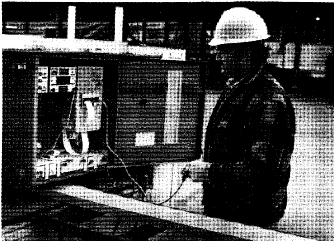
Calibration of a continuous lumber testing machine is an important aspect of overall quality control. This MSR machine separates high strength material for use in engineered wood structures (i.e., trusses, laminated beams).
