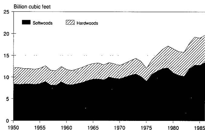
Figure 20.—Roundwood consumption, by species group, 1950–1986.
