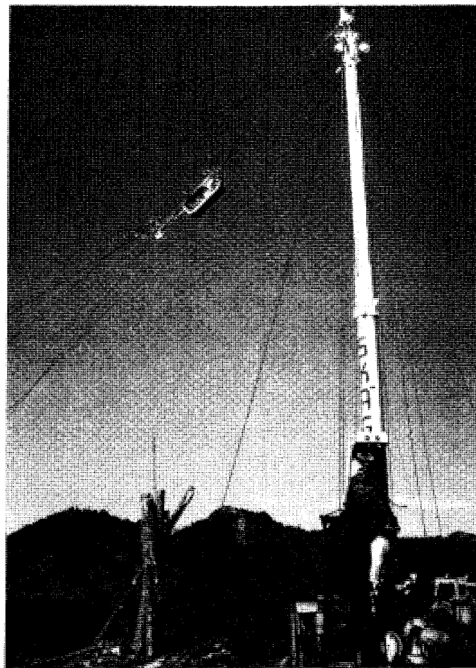
A Skagit tower with a high lead carriage system being used in steep terrain.
