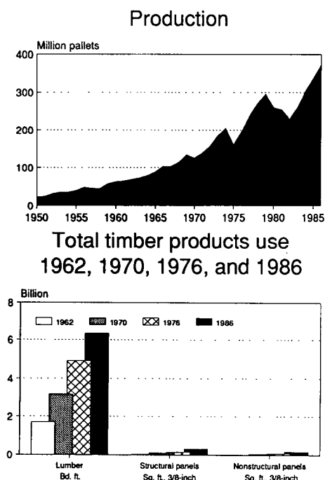
Figure 9.—Wooden pallets.
