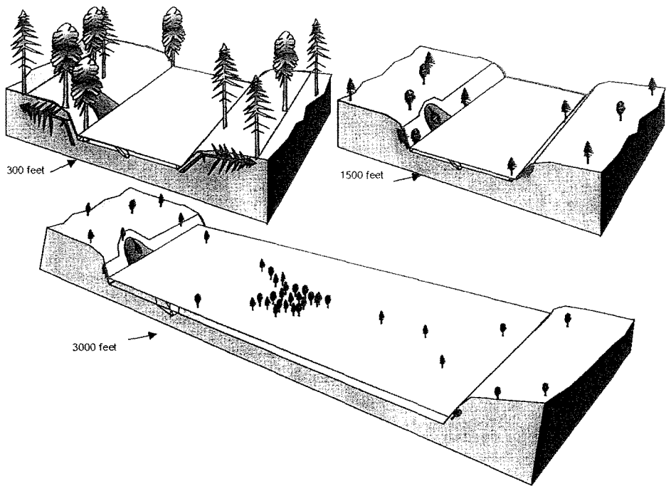
Figure 9. Floodprone area and its width are surveyed at an elevation that is twice the maximum bank-full channel depth (measured at a straight riffle section of the stream). The width of the floodprone area plus 100 ft (30 m) on either side provides a consistent, on-the-ground method to survey the attributes of riparian ecotones in any landscape. Including a 50 ft- (15 m)-wide band around known landslides or slumps completes riparian ecotone delineation. This recognizes their large impact on sediment flux in the channel.
