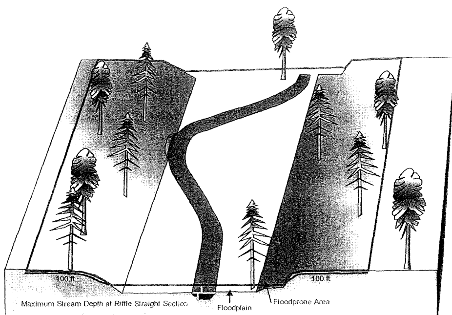
Figure 8. Twice the vertical distance from the thalweg (deepest part of a channel measured at a riffle section) to the bankfull elevation marks the elevation of the floodprone area (note the two vertical gray lines in the channel in the lower diagram). Floodprone areas are outlined and shown as a transparent plane above the stream and its floodplain. In flat valleys like these, there is not much difference in the area covered by a 25- or 50-year flood. The floodprone areas can be viewed as valleys carrying floodwater every 25 years or so, just as channels carry bankfull flows every year and a half or so.
