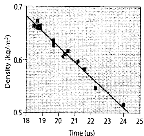
Fig.3. AU transmission time versus density for particleboard (control). AU transmission time was measured in propagation through thickness.
