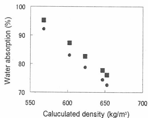
Fig. 4. Calculated density versus water absorption for particleboard (control). ■: 16.5 h, ●: 6.5 h. Density was determined from AU transmission time refereed to Fig. 3.
