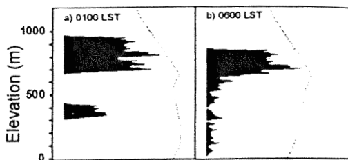
Figure 7. Vertical distribution of modeled insects during the transport phase.
