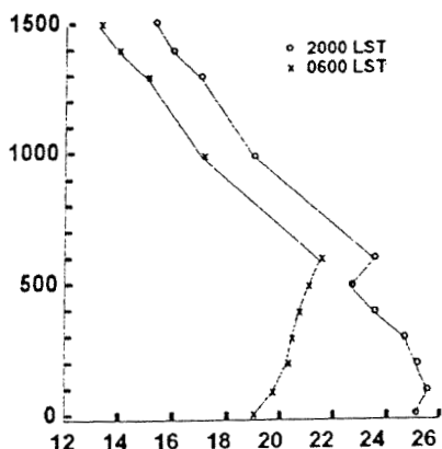
Figure 5. Schematic temperature sounding along insect migration pathway near sunset (circles) and near dawn (x's).
