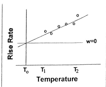
Figure 3. A possible insect rise rate/temperature relationship.
