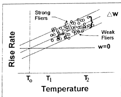
Figure 4. Same as Figure 3 but for an ensemble of insects.
