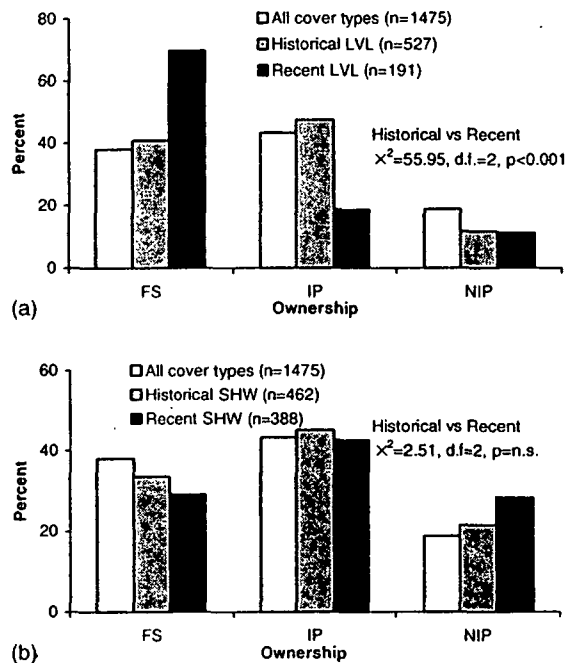
Fig. 2. Percent of total (a) large and very large conifer cover and (b) shrub and hardwood cover, in relation to land ownership class and time period. Percent distribution of ownership classes for the entire landscape (all cover types) is also shown. Percent is relative to the total amount within each class (e.g., historical LVL, etc.). Results of Chi-square tests for differences in distribution between dates are shown with each graph.
