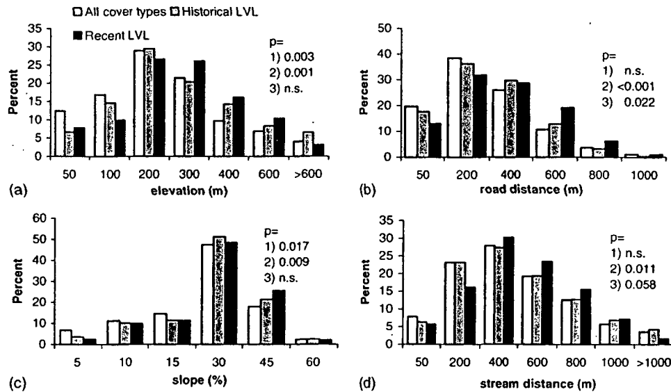
Fig. 3. Percent of total large and very large conifer cover in relation to (a) elevation, (b) road distance, (c) slope, and (d) stream distance historically and at recent times. Percent distribution of environmental classes and road distance for the entire landscape (all cover types) is also shown. Percent is relative to total amount within each class (e.g., historical LVL). Legend for all graphs is in graph a. P -values accompanying each graph are from Kolmogorov-Smirnov tests of difference between cover type distributions for (1) historical LVL vs. all; (2) recent LVL vs. all; (3) historical vs. recent LVL.
