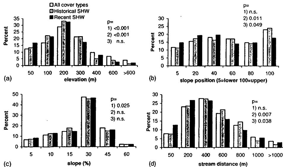
Fig. 4. Percent of total shrub and hardwood cover in relation to (a) elevation, (b) slope position, (c) slope, and (d) stream distance historically and at recent times. Percent occurrence of environmental classes for the entire landscape (all cover types) is also shown. Percent is relative to total amount within each class (e.g., historical SHW, etc.). Legend for all graphs is in graph a. P -values accompanying each graph are from Kolmogorov-Smirnov tests of difference between cover type distributions for (1) historical SHW vs. all; (2) recent SHW vs. all; (3) historical vs. recent SHW.
