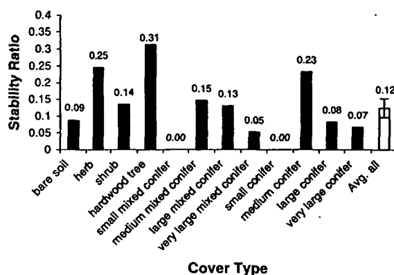
Fig. 5. Stability ratio of cover types. Ratio is proportion of historical (1939) plots that was the same cover type in 1993.
