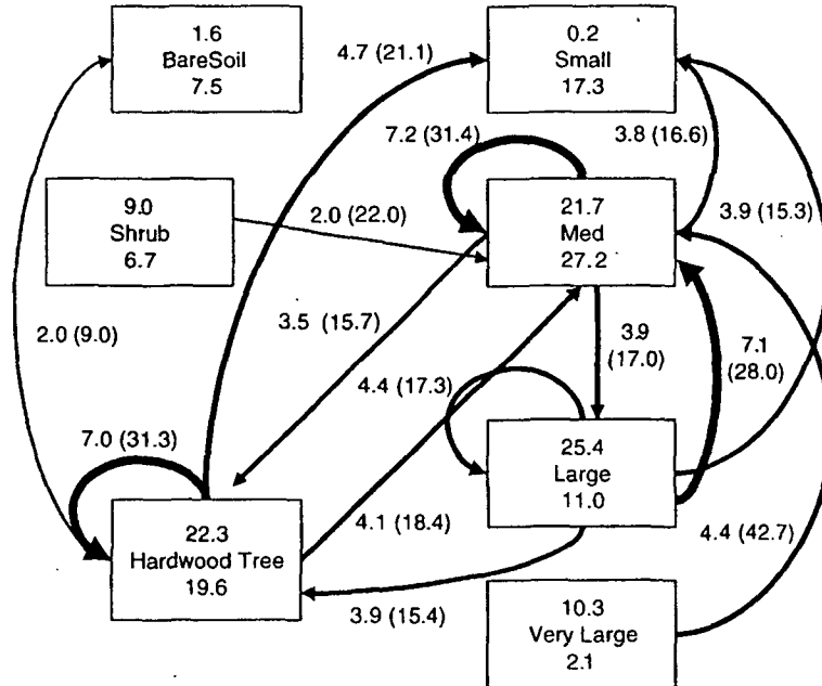
Fig. 6. Major landscape pathways from the early logging landscape (1939) to the recent modern forest management period (1993). All transitional pathways with >2.0% of all landscape plots ( n = 1475 ) are shown (shown n = 913 ; 62% of all plots). Arrow thickness is proportional to relative occurrence of pathway, and numbers with arrows are percent of all plots that followed that pathway and, in parentheses, the percent of the source cover type that followed that pathway. Numbers above and below cover types in boxes are, respectively, historical (1939) and recent (1993) total percentages of the landscape in that cover type.
