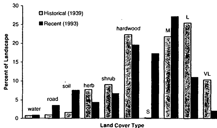
Fig. 1. Percent of land cover type in landscape, by date. S, M, L, and VL are size classes of combined mixed conifer and pure conifer cover types.
