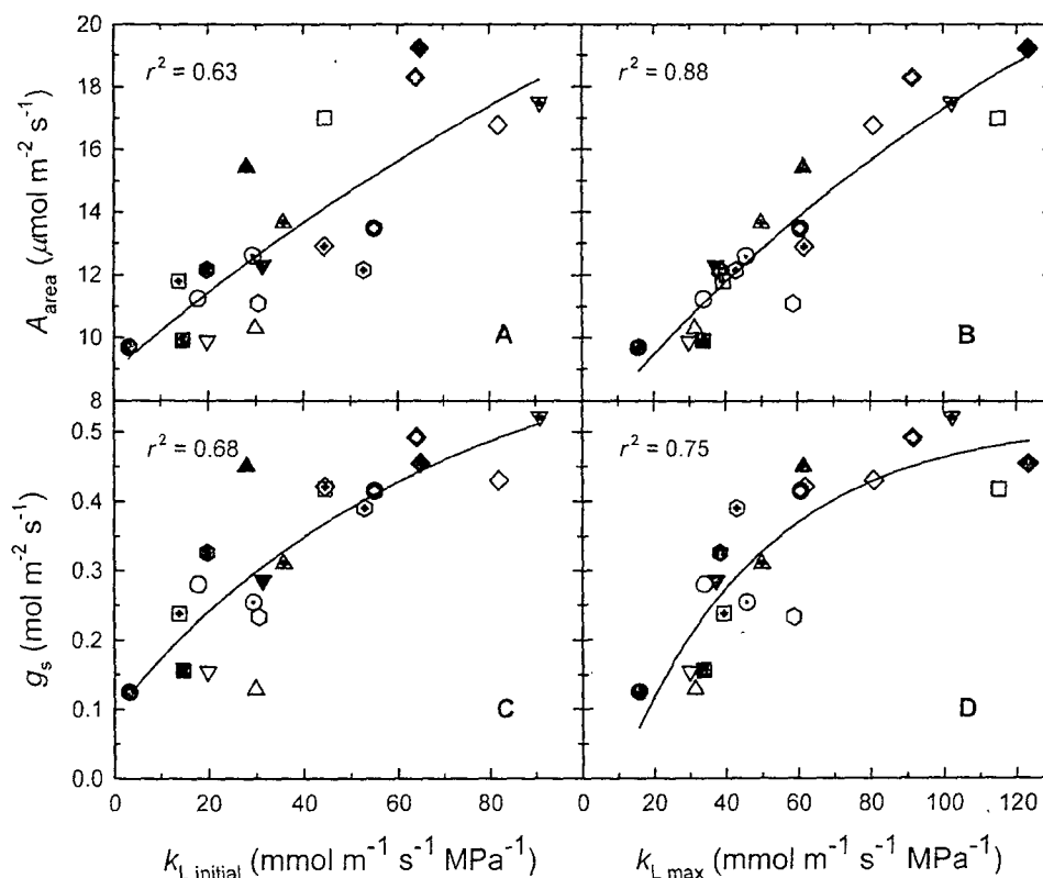
Fig. 1a–d Leaf photosynthetic rate per unit area ( A_{\text{area}} ; a, b) and stomatal conductance ( g_s ; c, d) as a function of initial and maximum leaf specific hydraulic conductivity ( k_L ) for 20 canopy tree species of lowland tropical forest in Panama. Values are species means. The solid lines represent best-fit non-linear regressions. A. cruenta (filled circle), C. cainito (filled square), C. alliodora (filled triangle), D. munda (filled inverted triangle), F. insipida (filled diamond), G. dumentorum (filled octagon), H. diguense (open circle), L.
