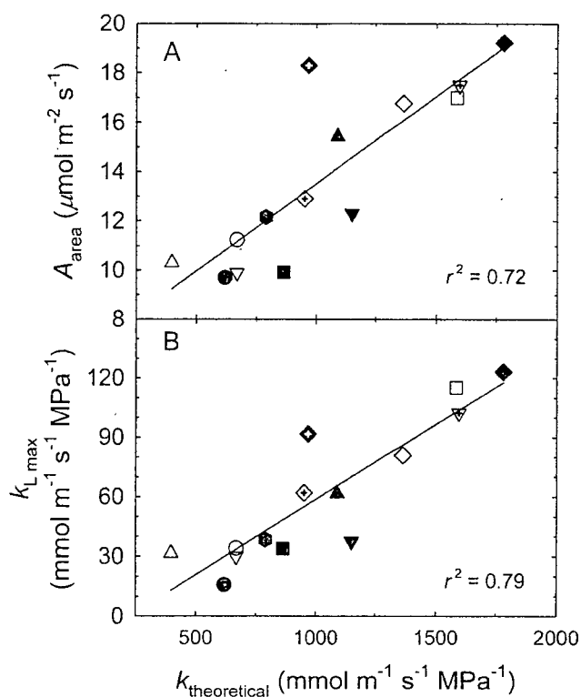
Fig. 3 a Maximum photosynthetic rate per unit area ( A_{\text{area}} ). b Maximum hydraulic conductivity per unit leaf area ( k_{L \text{ max}} ) and as a function of hydraulic conductivity per unit stem xylem area based on anatomical calculations ( k_{L \text{ theoretical}} ) for 14 species of lowland forest canopy trees in Panama. Values are species means. The solid lines represent best-fit linear regressions. Symbols as in Fig. 1
