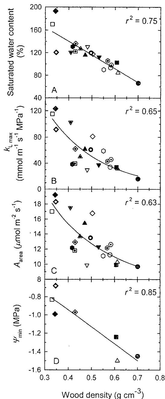
Fig. 4 a Stem saturated water content. b Maximum leaf specific hydraulic conductivity ( k_L max). c Photosynthetic rate per unit leaf area ( A_{area} ). d Minimum water potential ( \Psi_{min} ) measured on covered leaves as a function of stem wood density for lowland forest canopy trees in Panama. Values are species means. The solid lines represent best-fit linear and non-linear regressions. Symbols as in Fig. 1
