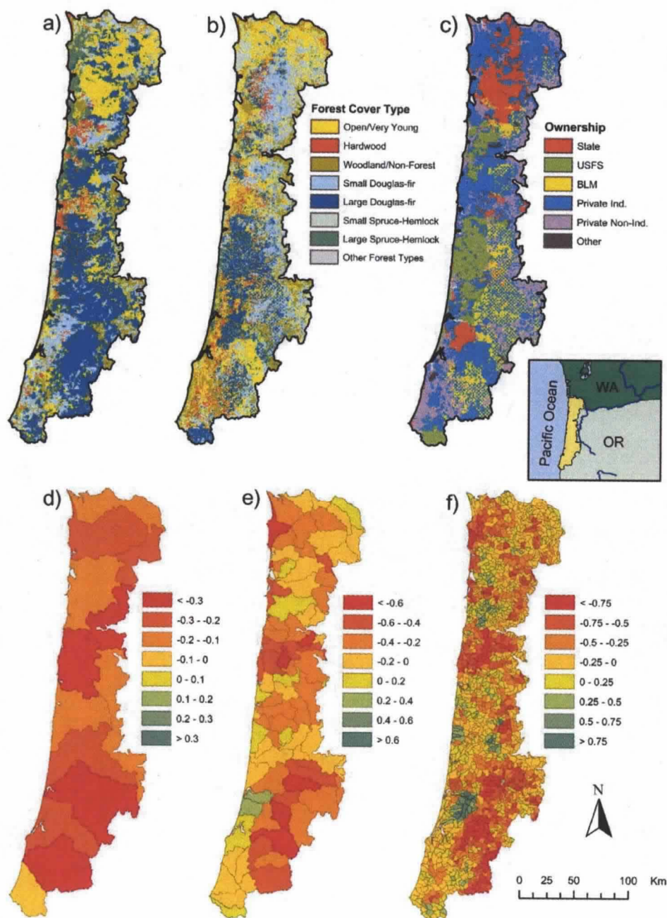
Figure 1. Changes in the pattern of forest cover types in the Oregon Coast Range from 1936 to 1996. (a) 1936 pattern of forest cover types; (b) 1996 pattern of forest cover types; (c) major land ownership classes; (d) LCCHNG summarized by subbasin; (e) LCCHNG summarized by watershed; (f) LCCHNG summarized by subwatershed.
