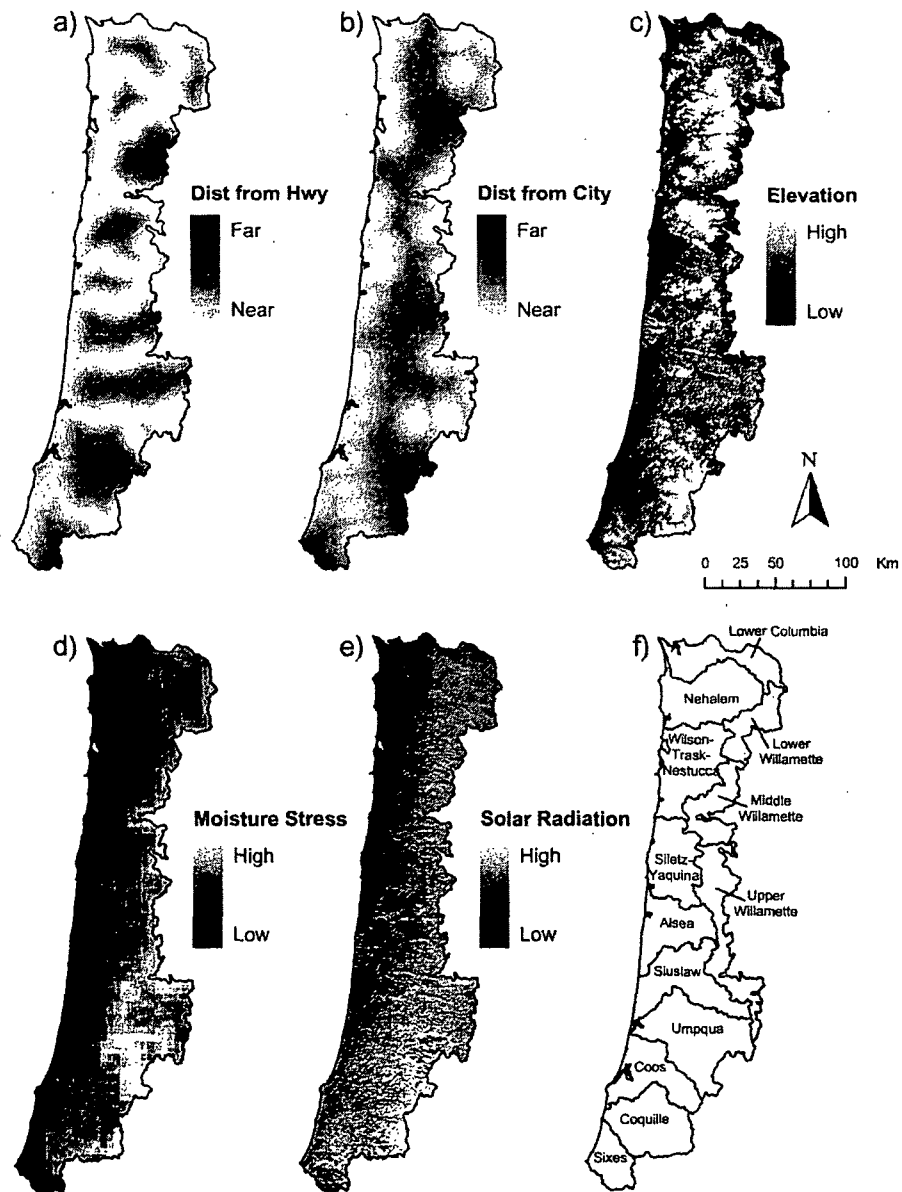
Figure 2. Independent variables used to model forest land cover change in the Oregon Coast Range. (a) Distance from the nearest highway; (b) Distance from the nearest city; (c) Elevation (used to compute topographic relief); (d) Moisture stress index; (e) Solar radiation (see Table 2 for additional details); (f) names and locations of the 13 subbasins used to summarize land cover change in Table 4.
