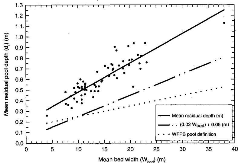
Fig. 3. Increase in mean residual pool depth with channel bed width, showing our proposed revision to the WFPB (1993) minimum residual depth definition of a pool.
