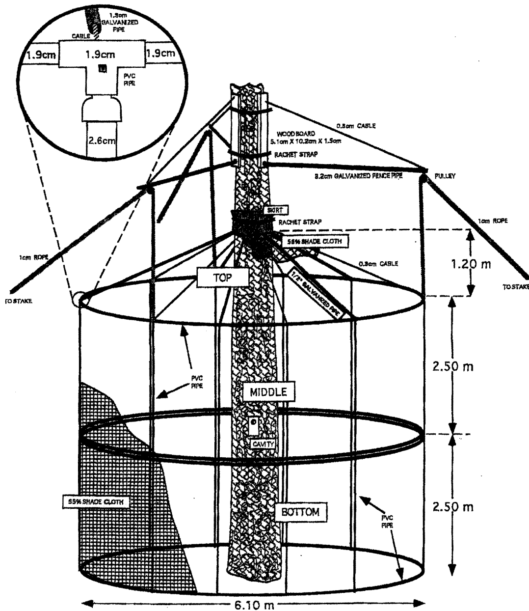
Figure 1. Diagram of mobile aviary designed for the red-cockaded woodpecker
