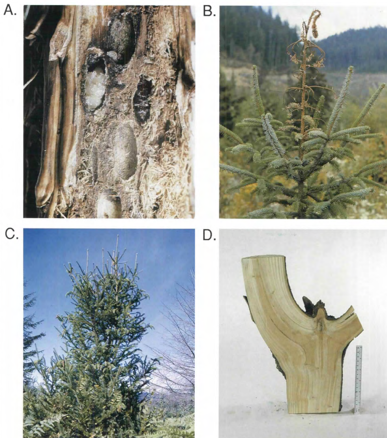
Figure 1—Damage to Sitka spruce by Pissodes strobi . A. Weevil larvae mine down the terminal shortly after bud burst and, in midsummer, form pupal cells under the bark at the end of the mines. B. New growth arising from attacked terminal dies and starts to droop when the mining larvae grow large enough to sever conductive tissue. C. Multiple tops often develop when laterals below the killed terminal assume dominance. D. Killed terminals overgrown by laterals-turned-to-leaders result in poor stem form and decreased wood quality.
