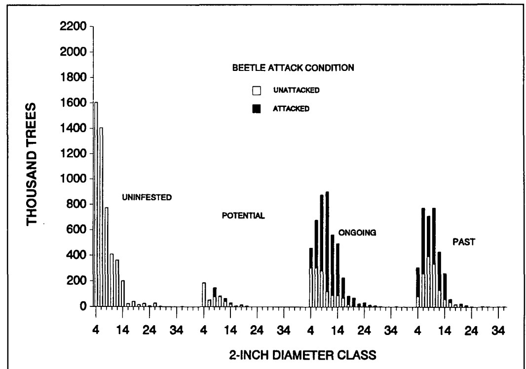
Figure 3—Estimated number of dead white spruce trees on timberland and "high-site" other forest land by stage of infestation, 2-inch diameter class, and condition of beetle attack, Kenai Peninsula, Alaska, 1987.
