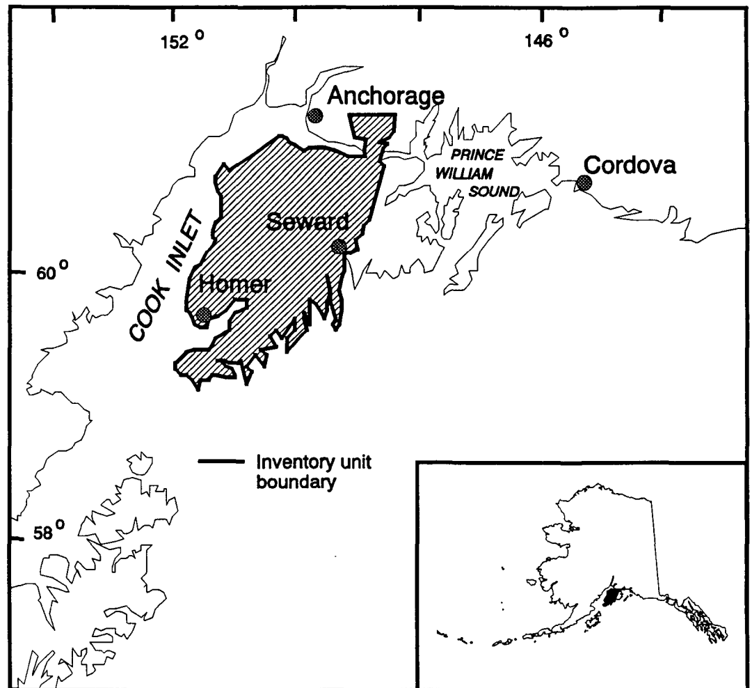
Figure 1—Study area, Kenai Peninsula, Alaska, 1987.
