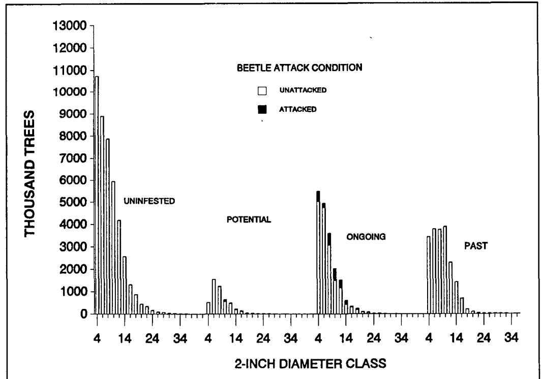
Figure 2—Estimated number of live white spruce trees on timberland and "high-site" other forest land by stage of infestation, 2-inch diameter class, and condition of beetle attack, Kenai Peninsula, Alaska, 1987.
