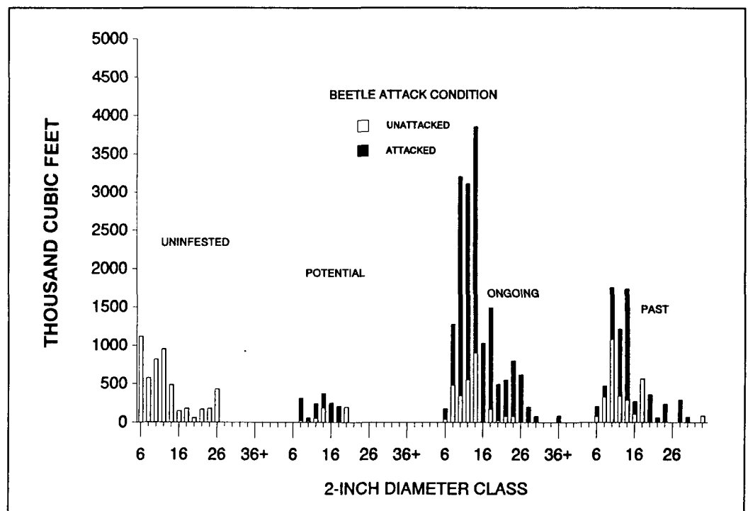
Figure 5—Estimated gross cubic-foot volume in dead white spruce trees on timberland and "high-site" other forest land by stage of infestation, 2-inch diameter class, and condition of beetle attack, Kenai Peninsula, Alaska, 1987.
