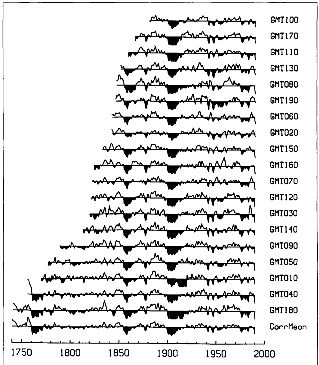
Figure 6—Corrected tree-ring index chronologies (averages of two cores per tree) from grand fir in the Green Mountain stand. The lowermost plot is the stand chronology; that is, the average of all the tree chronologies.
