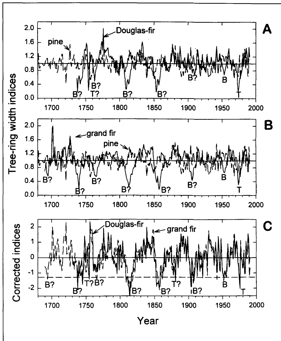
Figure 3—Overlay plots of the Grizzly Bear Meadow Douglas-fir and grand fir tree-ring index chronologies and the Cross Canyon ponderosa pine chronology (parts A and B). Sharply reduced growth periods in the Douglas-fir and grand fir are visible corresponding to known and inferred outbreaks of western spruce budworm (B) and Douglas-fir tussock moth (T). Inferred outbreaks are shown with a question mark. Part C shows the corrected tree-ring indices (standard deviation units) for the Douglas-fir and grand fir, produced by subtracting a rescaled version of the pine chronology. The dashed horizontal line is the 1.28 standard deviation threshold. Not all possible outbreaks, based on the threshold, are obvious in the overlay comparisons (A and B), but they appear more clearly in the corrected version (C).
