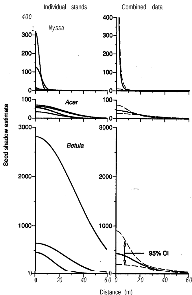
Fig. 10. Seed shadow estimates for individual stands (left-hand side) and for data from all stands simultaneously (right-hand side). Dashed lines on right are 95% confidence intervals determined by propagating parameter error and correlation (Clark, 1998). The seed shadow has units of seeds·m -2 ·yr -1 .
