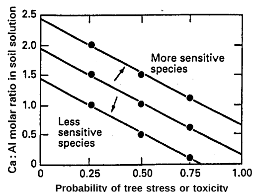
Fig. 10. A survey of forest responses to variations in the Ca:Al ratio in soil solutions has been used to develop generalized response surfaces that describe relative risks of impairment of forest processes by low Ca and high Al levels. Contrasts between mean, sensitive and more resistant species are noted (Cronan & Grigal, 1995).
