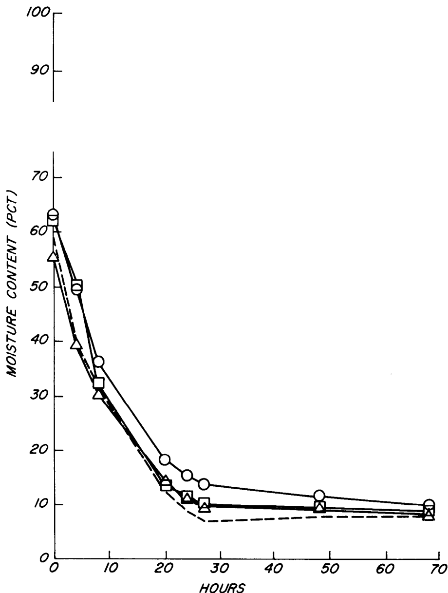
Figure 6.—Drying curves for Trial Schedule V. (M 148 461)
