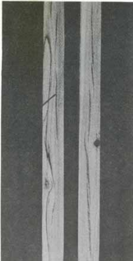
Figure 3.—Severe honeycomb in heartwood of studs sawn from flitches dried by Trial Schedule II. (M 147015)
