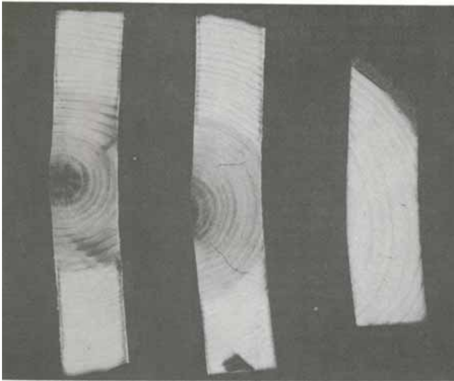
Figure 1.—Typical cross section of flitches dried by Trial Schedule I. (M 147016)
