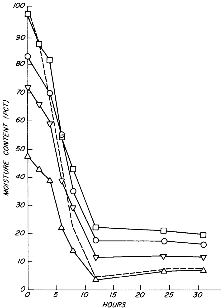
Figure 4.—Drying curves for Trial Schedule III. (Note large spread in initial MC and at end of run.). (M 148 462)
