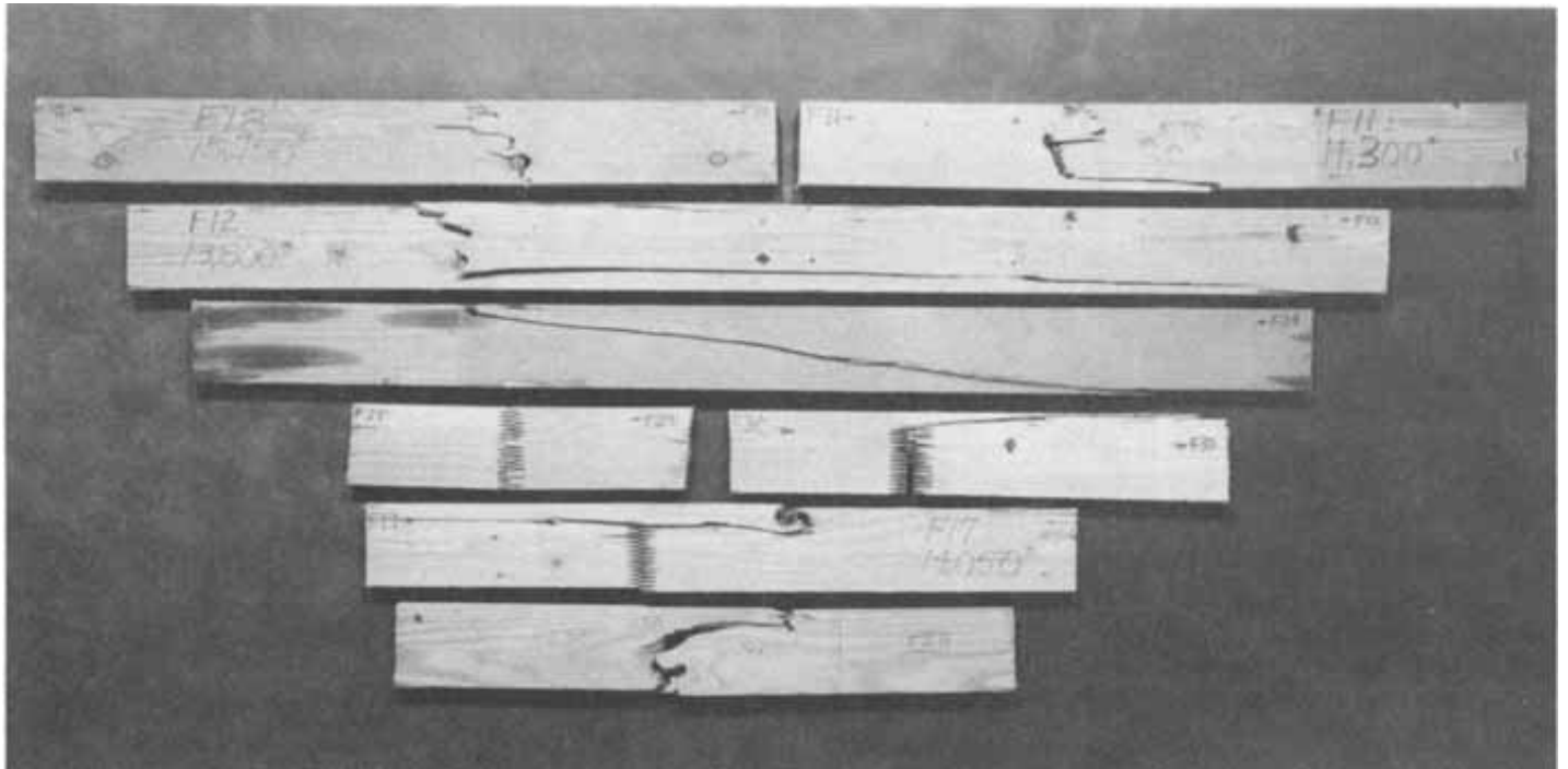
Figure A-7.—Most of these 302-24 DF-L beam failures occurred at a level slightly above the target level. Beam F23 failed below the target level. (M 147 126)
