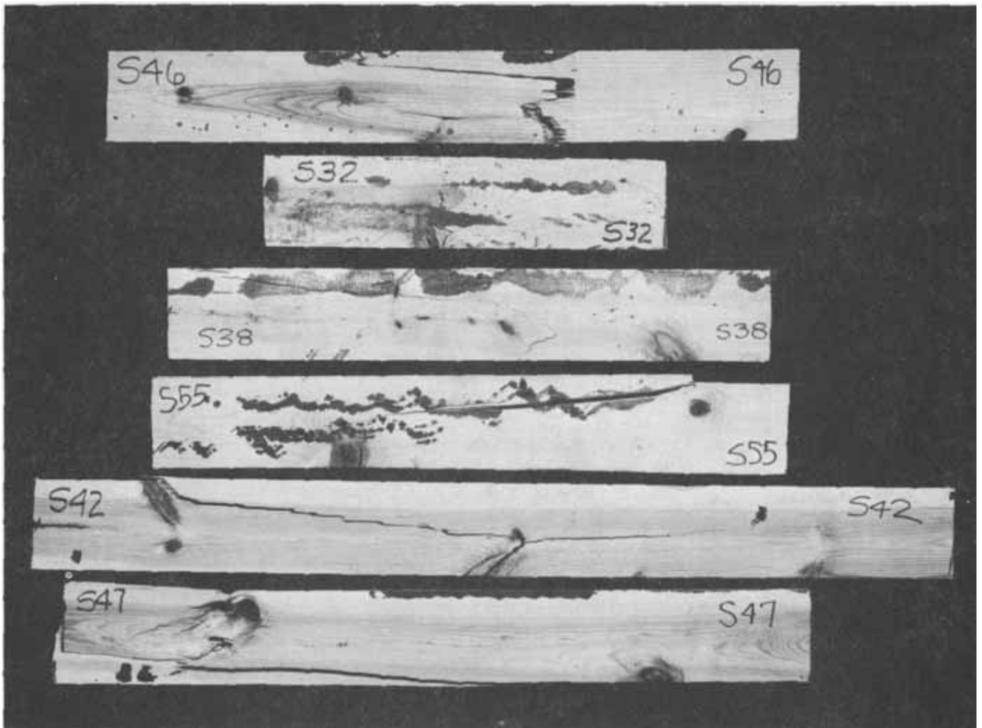
Figure A-5.—Failure sections of the beams from the second set of No. 1D SP beams that failed more than 15 percent below the target MOR level. (M 147 310)
