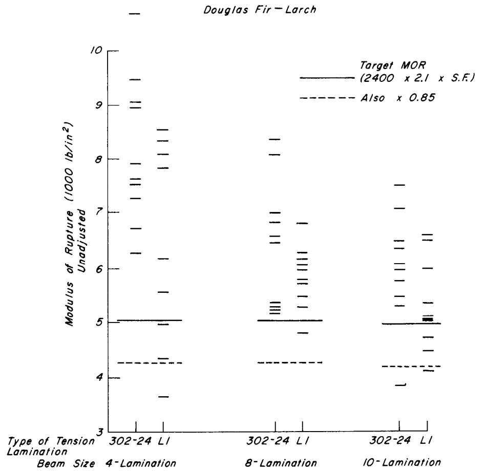
Figure 8.—Comparison of the DF-L test MOR values with the appropriate target MOR value.
