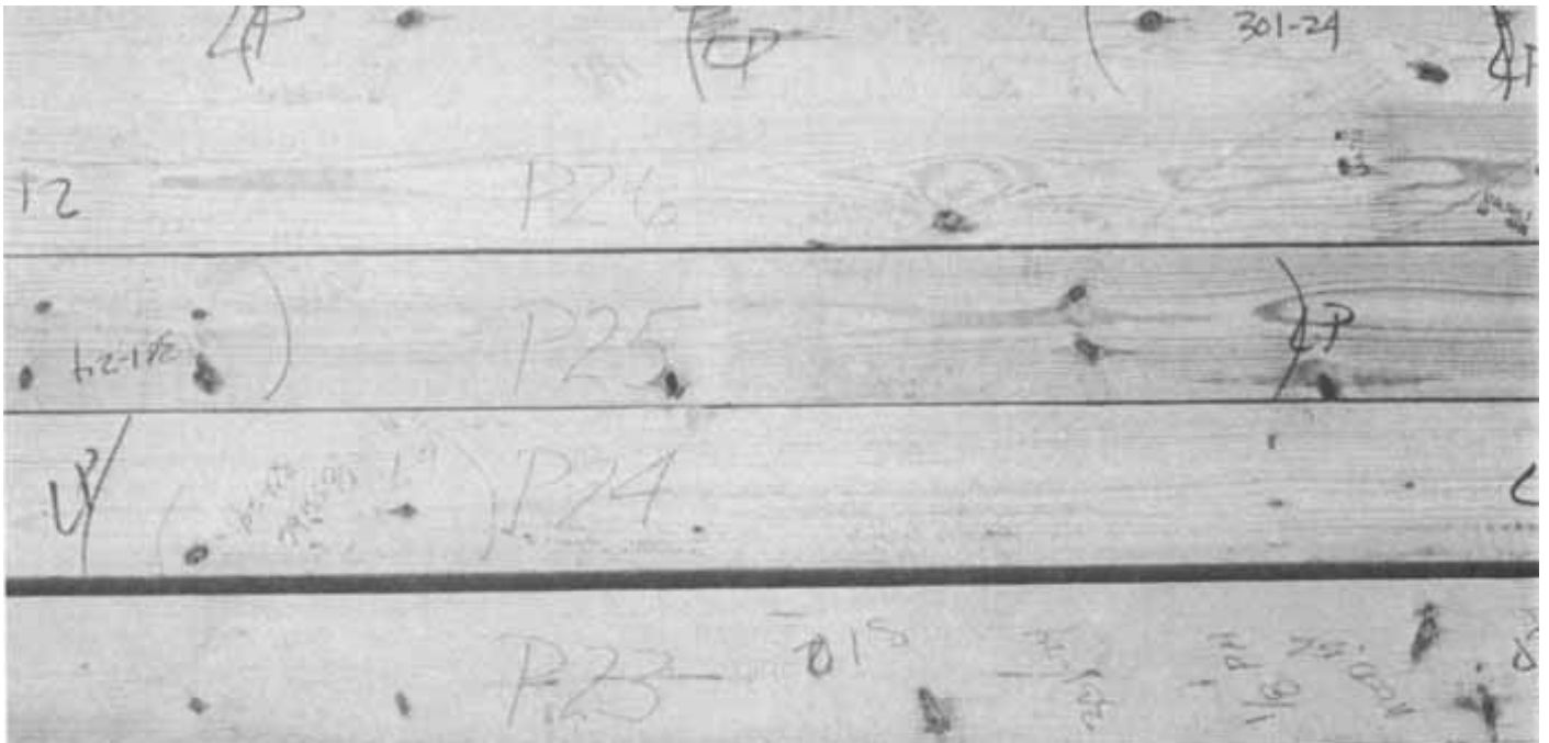
Figure 2.—Some 302-24 SP boards that illustrate the quality of 302-24 tension laminations selected for this study.
