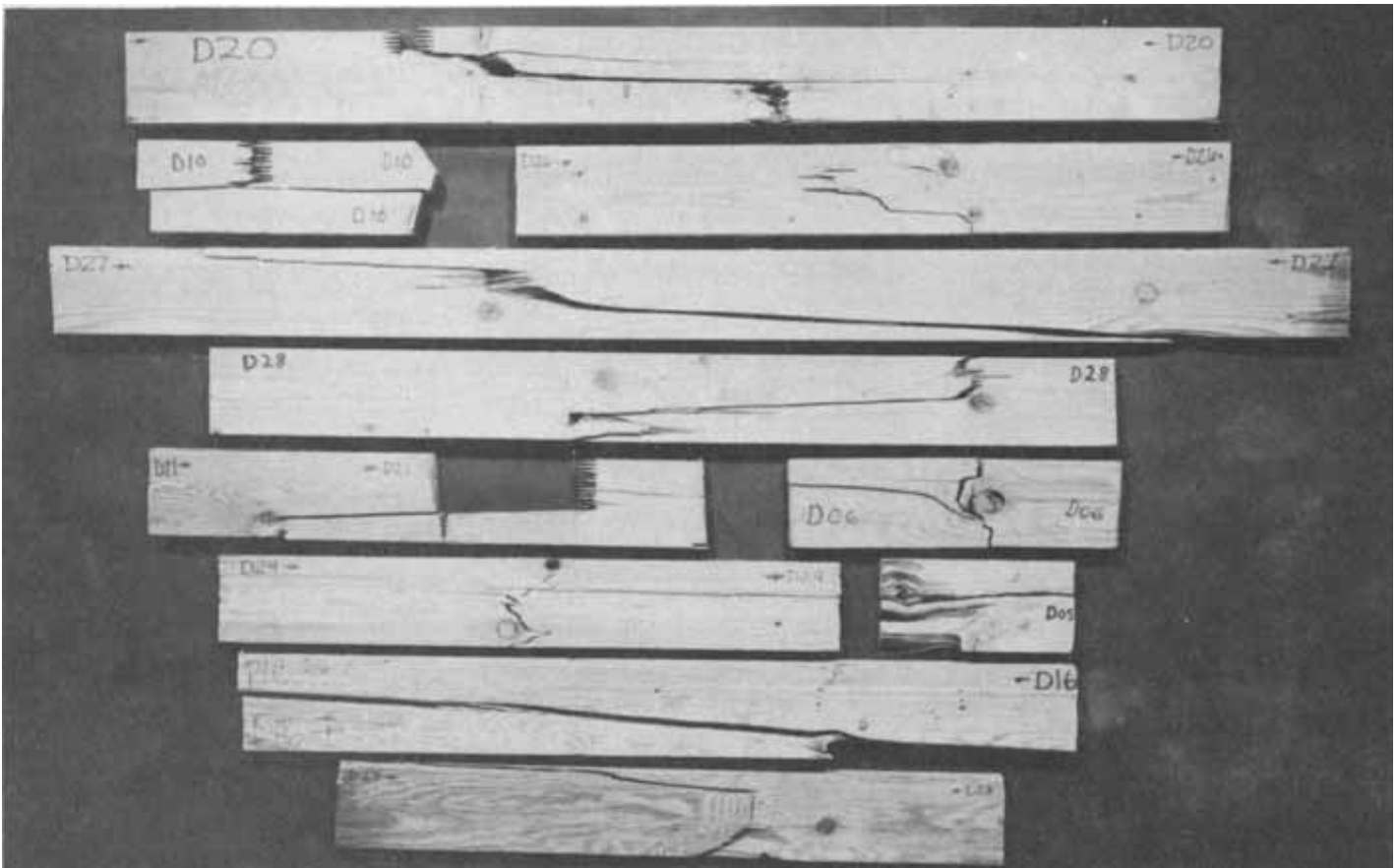
Figure A-9.—All of the below-target L1 DF-L beam failures are shown here along with some selected failures just above the target level. The photograph also illustrates the typical, near-minimum quality of L1 tension laminations selected. (M 147 138)
