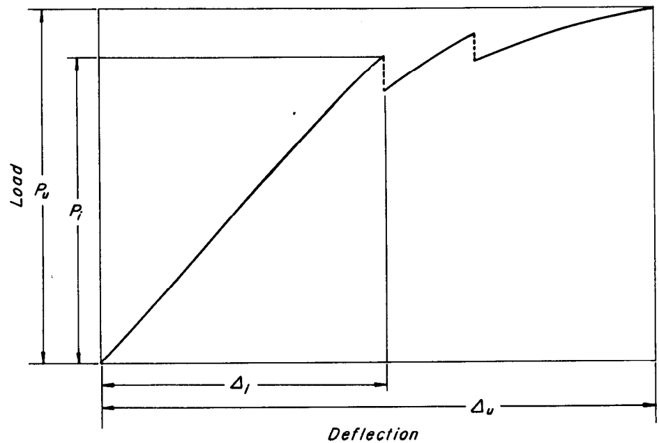
Figure A-10.—A typical example of a load versus deflection curve for a beam that failed gradually. Load ( P_i ) and deflection ( \Delta_i ) at first failure are shown along with ultimate load ( P_u ) and deflection ( \Delta_u ). The slope of the initial P-A curve is the basis for calculating the modulus of elasticity (MOE). (M 148953)
