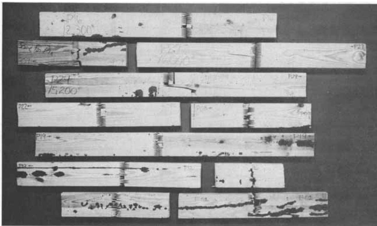
Figure A-1.—Failure sections of the initial set of 302-24 SP beams that failed below the target MOR level. (P18 is missing from the photograph.) Also illustrated is the typical appearance of the initial 302-24 SP finger-joint failures.
