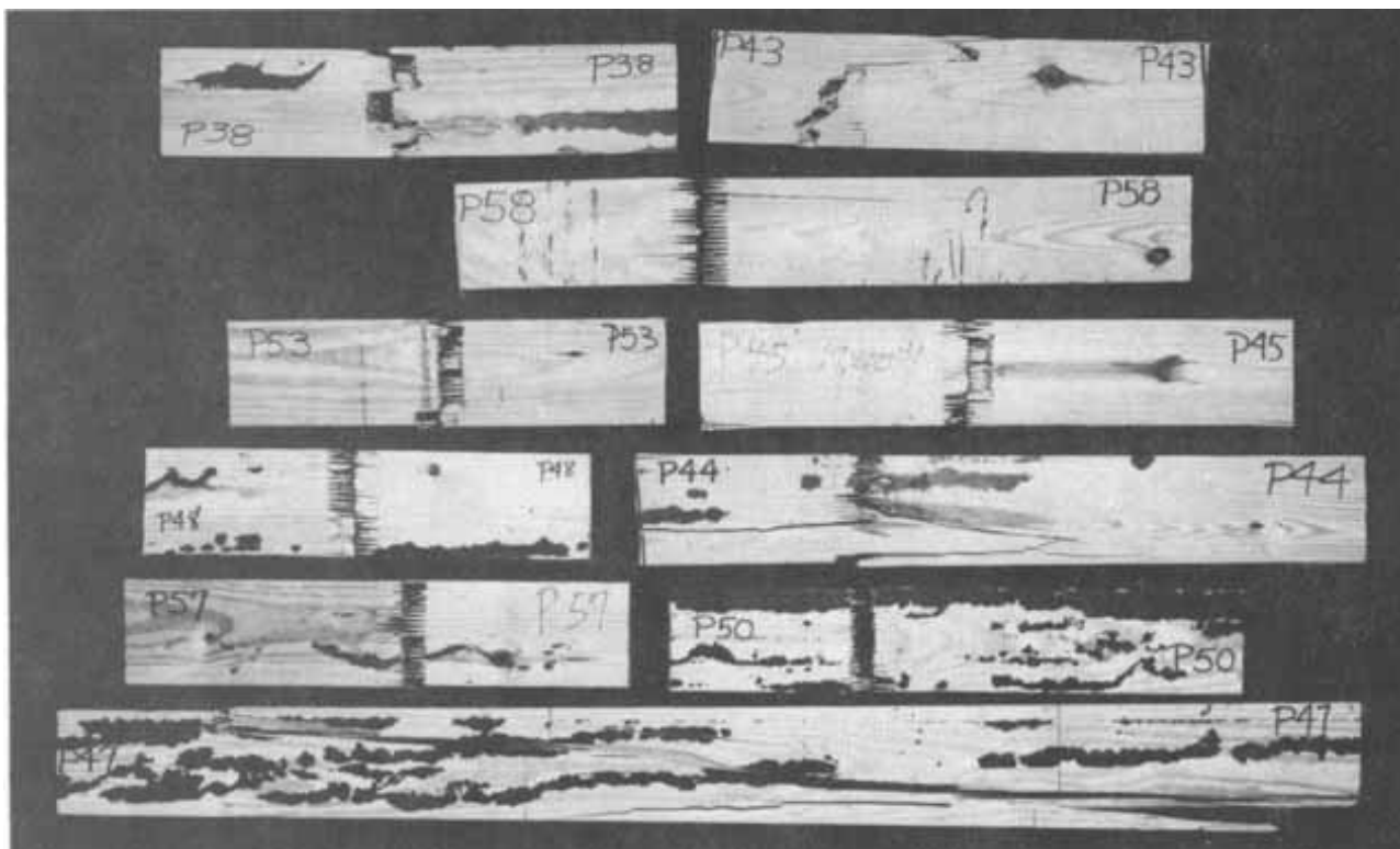
Figure A-4.—Failure sections of the beams from the second set of 302-24 SP beams that had a finger joint involved in the failure, Also illustrated is the typical appearance of the second set of SP finger-joint failures. (M 147 312)
