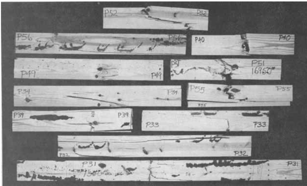
Figure A-3.—Selected failures from the second set of 302-24 SP beams. P52 (top) was the Only beam that failed below the target MOR level. (M 147311)
