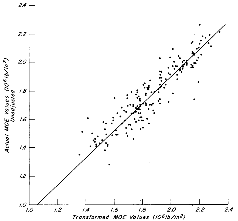
Figure 6.—Comparison of actual and transformed MOE values. Calculations for transformed values were based on actual stiffness of individual pieces of lumber used in the beams.
