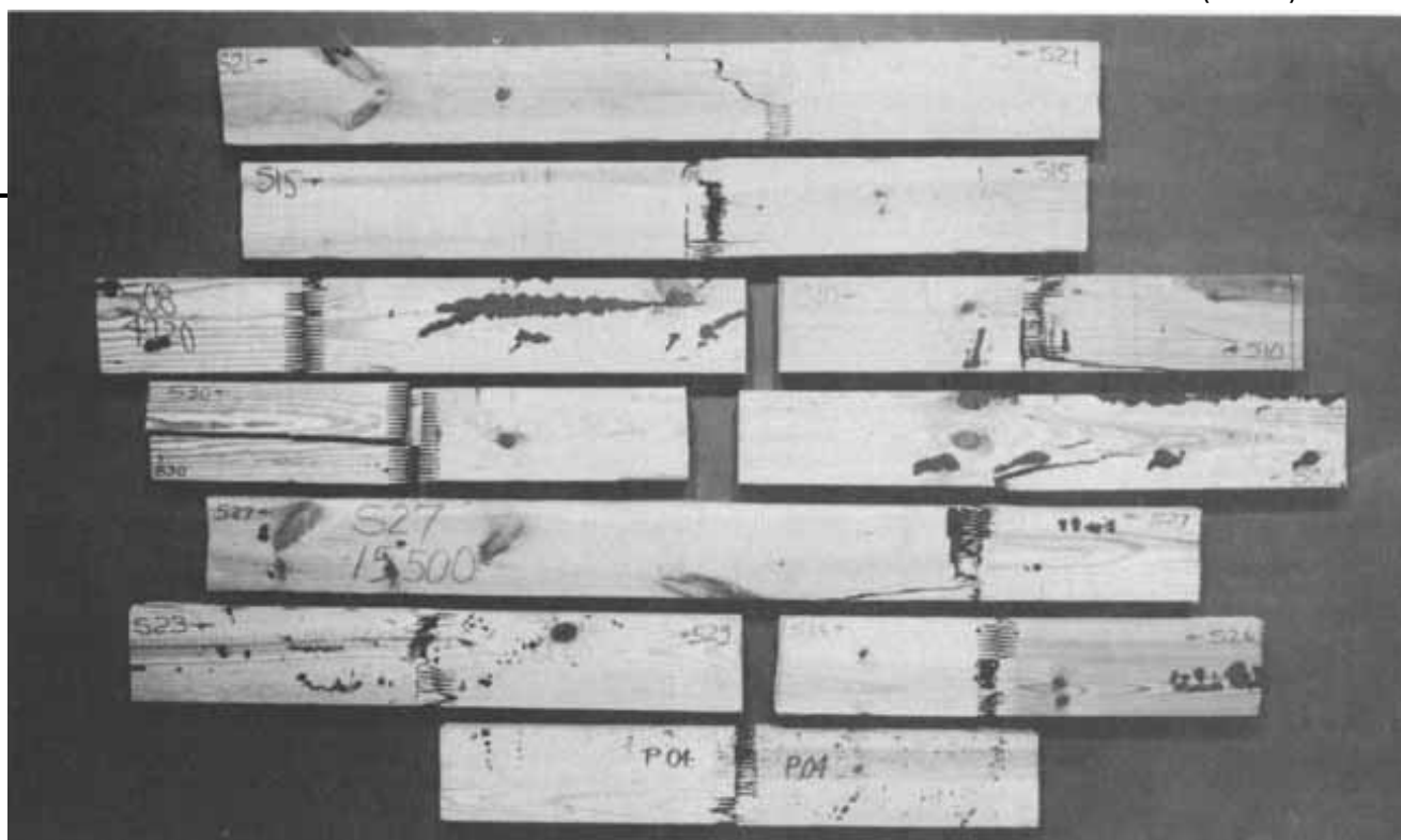
Figure A-2.—Failure sections of the initial set of No. 1D SP beams that failed below the target MOR level. (S20 is missing from the photograph.) Also illustrated is the typical appearance of the initial No. 1D finger-joint failures.
