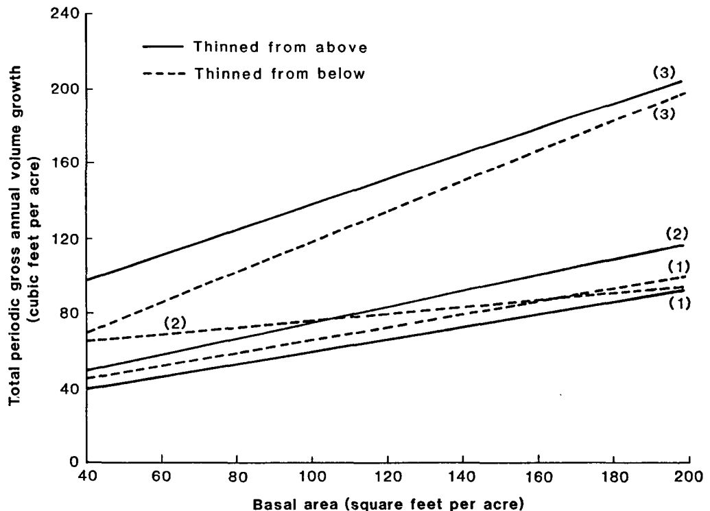
Figure 4—Total periodic gross annual cubic volume growth by thinning method and growth period as a function of stand density; numbers in parentheses are growth periods.
