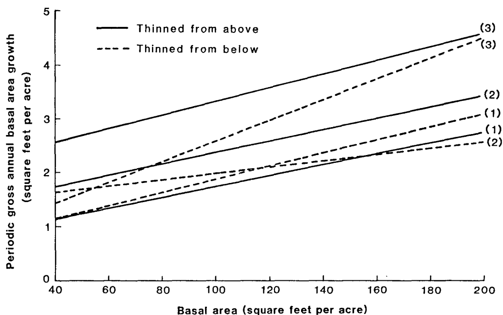
Figure 3—Periodic annual gross basal area growth by thinning method and growth period as a function of stand density; numbers in parentheses are growth periods.
