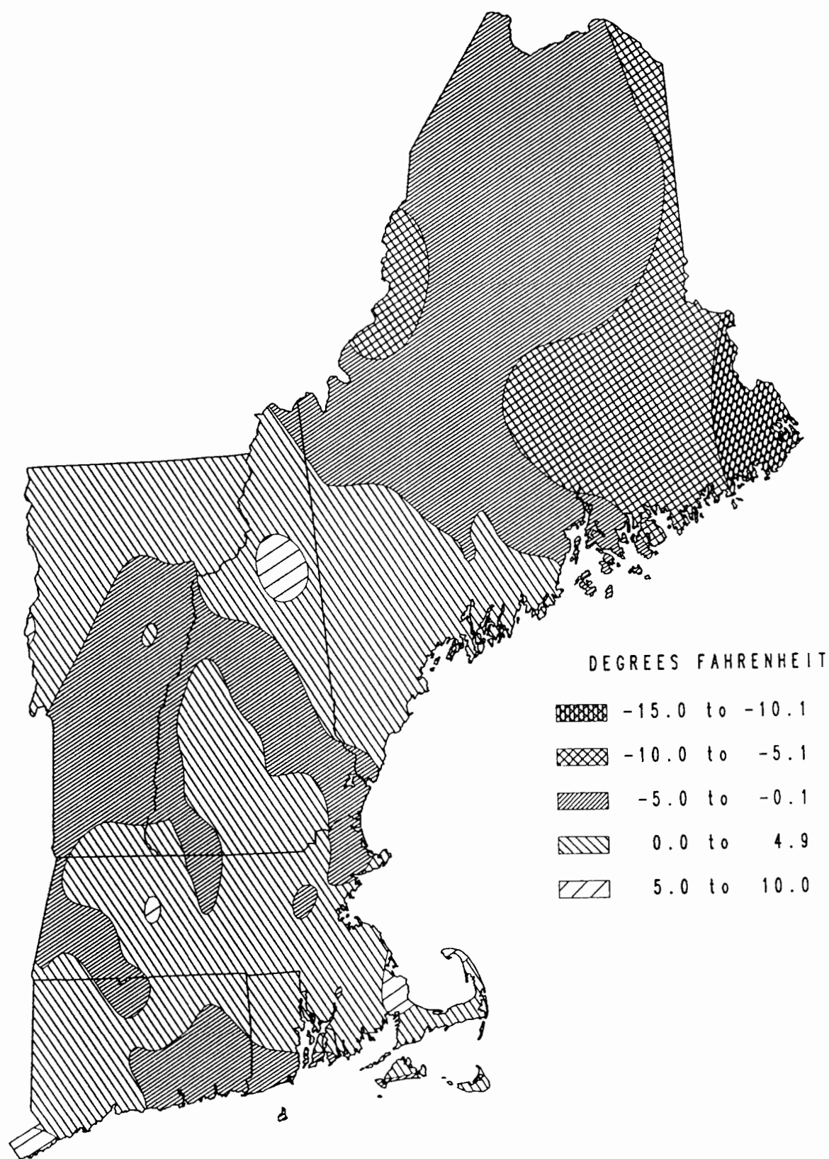
Figure 16.--Isopleth map of annual minimum temperature deviations from the 30-year average, New England, October 1989 through September 1990.
