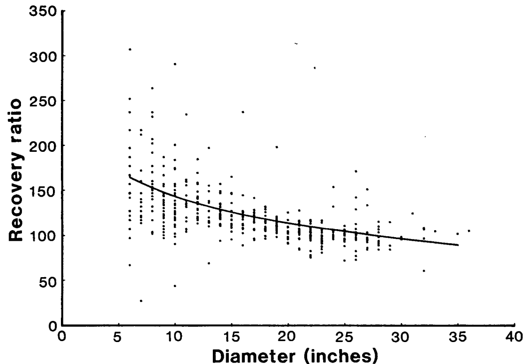
Figure 3.--Recovery ratio curve for all live ponderosa pine logs. (Recovery ratio = 106.7545 - 0.9471(D) + 568.3461(1/D) - 1116.9745(1/D^2) ). Coefficient of determination = 0.2533. Standard deviation from regression = 35.35.)
