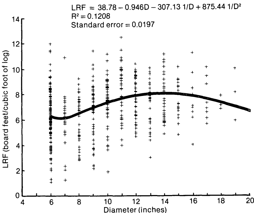
Figure 6. — Lumber recovery factor (LRF) — nominal board-foot volume of lumber recovered from each gross cubic foot of log processed — for young-growth red and white fir logs, by log scaling diameter.
