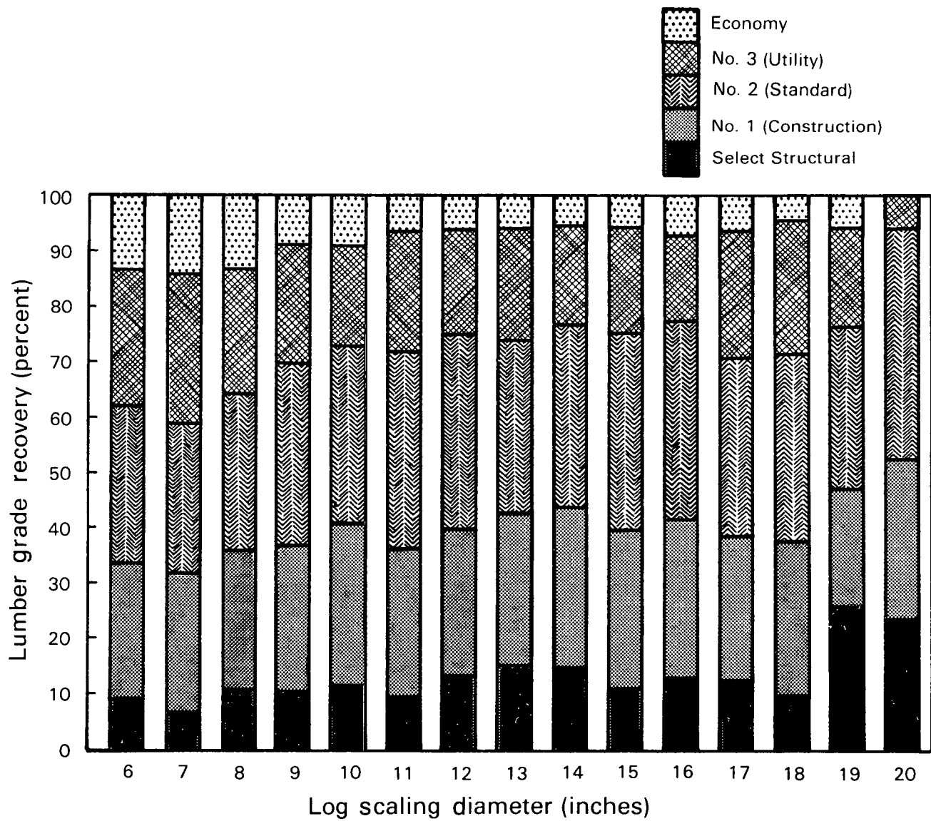
Figure 5. — Percent of lumber grade volumes recovered from young-growth red and white fir logs, by scaling diameter.
