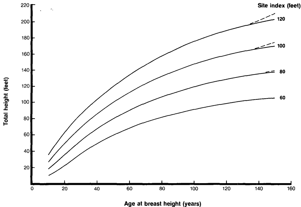
Figure 14.—Site index curves for unmanaged, even-aged Sitka spruce in southeast Alaska. Dashed lines connect decadal points derived from the unsmoothed basic data regressions of (S - 4.5 \text{ feet}) = a_2 + b_2 (HT - 4.5 \text{ feet}) . Solid lines represent smooth curves from a rearrangement of the estimating equation.
