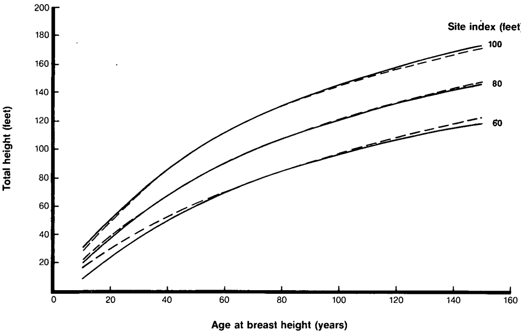
Figure 11.—Site index (solid lines) and height growth curves (dashed lines) for unmanaged, even-aged western hemlock in southeast Alaska.
