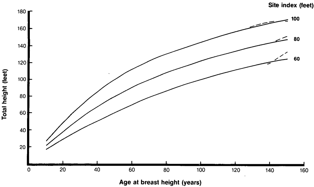
Figure 10.—Height growth curves for unmanaged, even-aged western hemlock in southeast Alaska. Dashed lines connect decadal points derived from the unsmoothed basic data regressions of (HT - 4.5 \text{ feet}) = c_1 + d_1 (S - 4.5 \text{ feet}) . Solid lines represent smooth curves from the estimating equation. Heights represent the means among the 40 largest diameter trees per acre.
