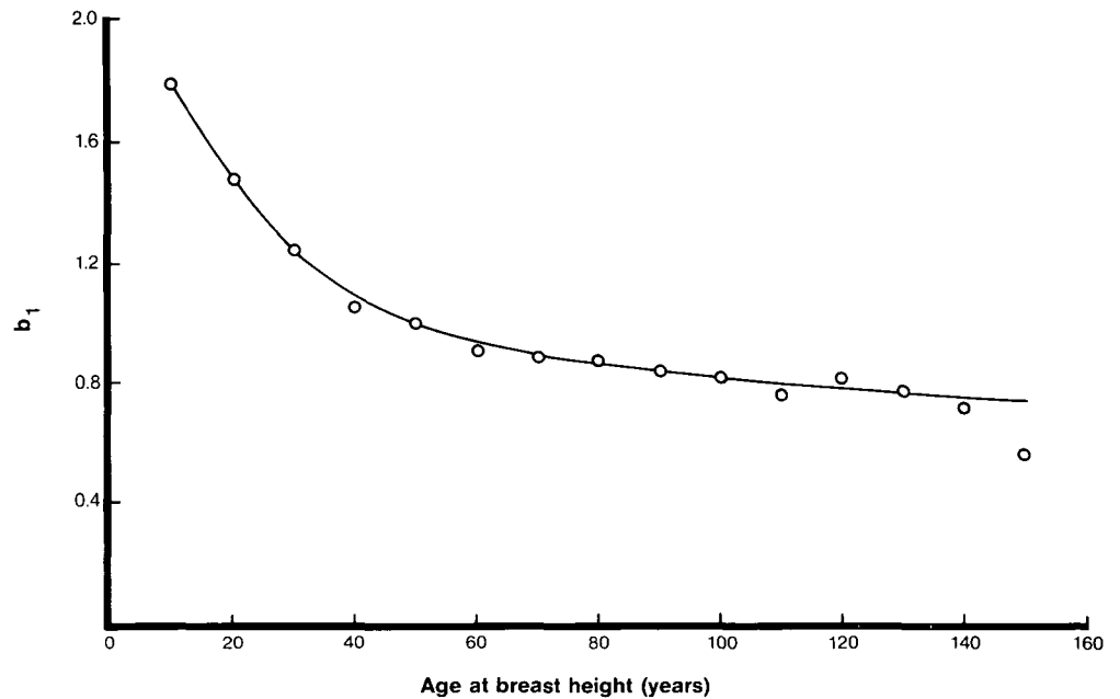
Figure 6.— b_1 values for western hemlock in the equation (S - 4.5 \text{ feet}) = a_1 + b_1 (HT - 4.5 \text{ feet}) as a function of age. Plotted points are actual b_1 values. Solid line is expressed by the equation \hat{b}_1 = e^{x_1} . Coefficient x_1 is defined in the text. Standard error is 0.00071 and r^2 is 0.9922.
