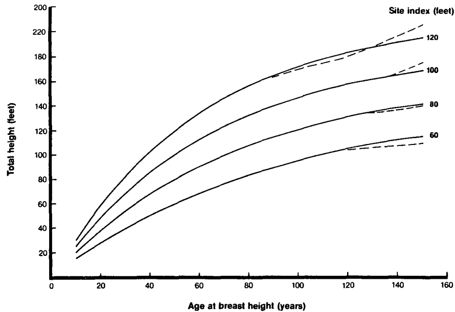
Figure 16.—Height growth curves for unmanaged, even-aged Sitka spruce in southeast Alaska. Dashed lines connect decadal points derived from the unsmoothed basic data regressions of (HT - 4.5 \text{ feet}) = c_2 + d_2 (S - 4.5 \text{ feet}) . Solid lines represent smooth curves from the estimating equation. Heights represent the mean among the 40 largest diameter trees per acre.
