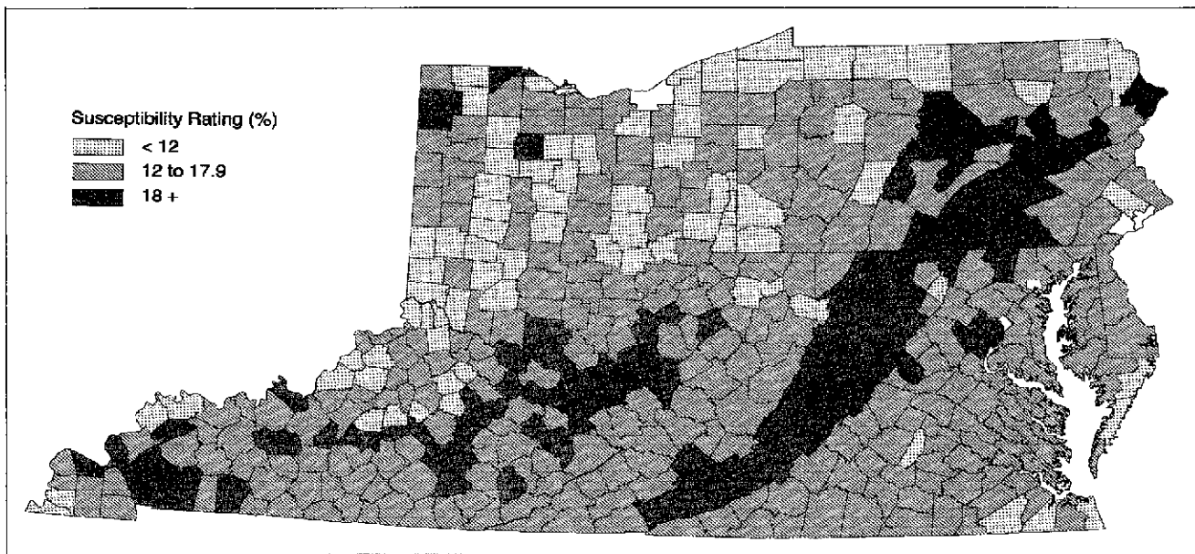
Figure 2.—Gypsy moth defoliation potential in seven threatened states, by county.
