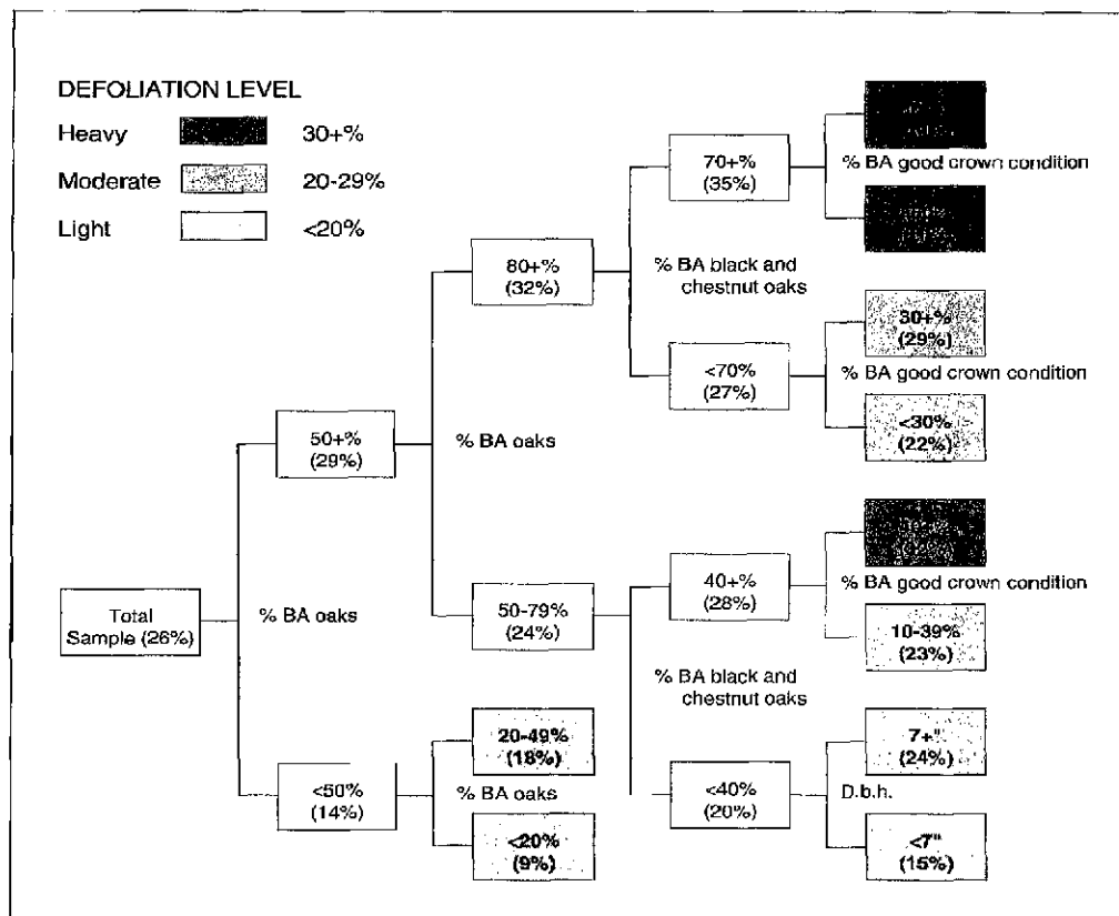
Figure 1.—Guide for estimating gypsy moth defoliation potential. Any hardwood stand can be assigned to a defoliation group on the basis of characteristics of the stand. The 3-year average defoliation percentage is shown in parentheses for each group.
