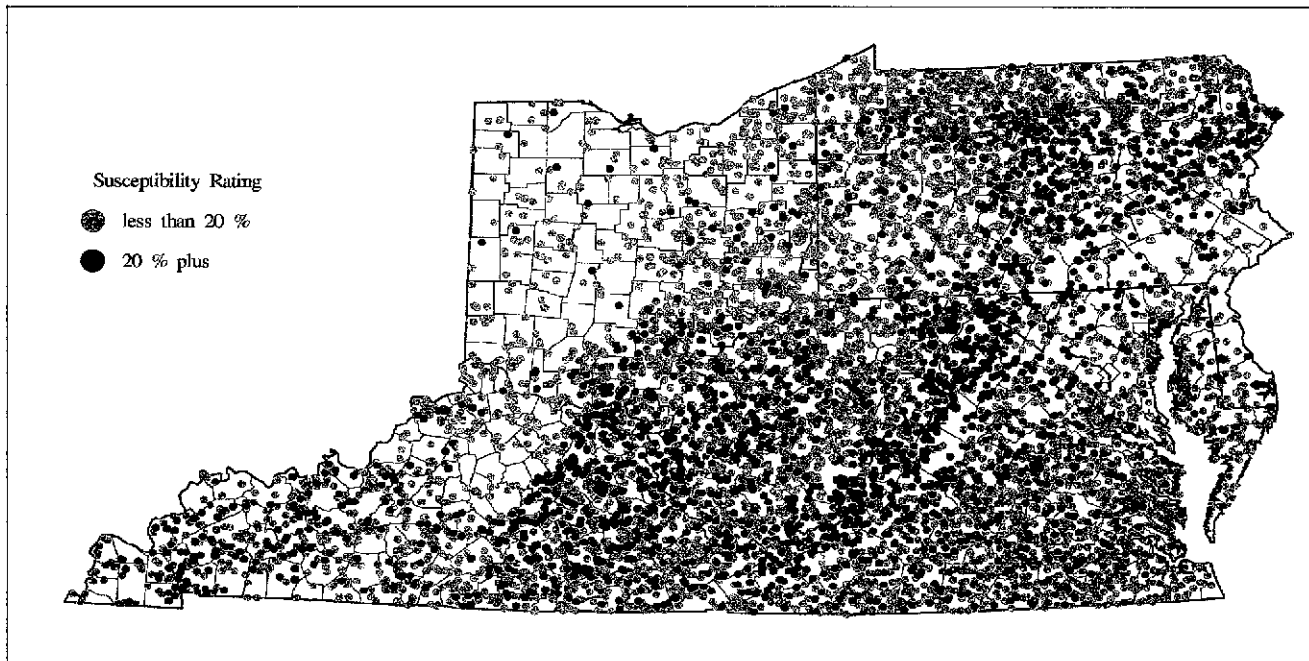
Figure 3.—Gypsy moth defoliation potential: each dot represents approximately 10,000 acres of forest land.
