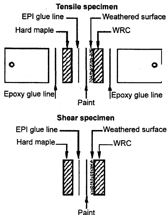
Figure 1. ~ Expanded view of tensile and shear specimens showing interphases.
