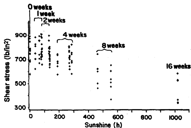
Figure 5. ~ Ultimate shear stress compared with sun-light exposure time of acrylic latex primer on WRC. Only primer/wood interphase failures are shown.
