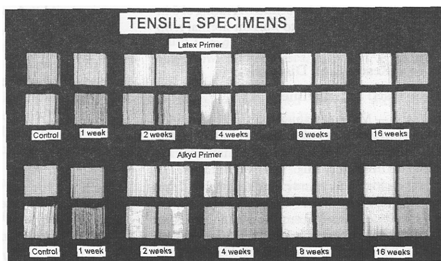
Figure 4. ~ Failure surfaces of representative tensile specimens.
