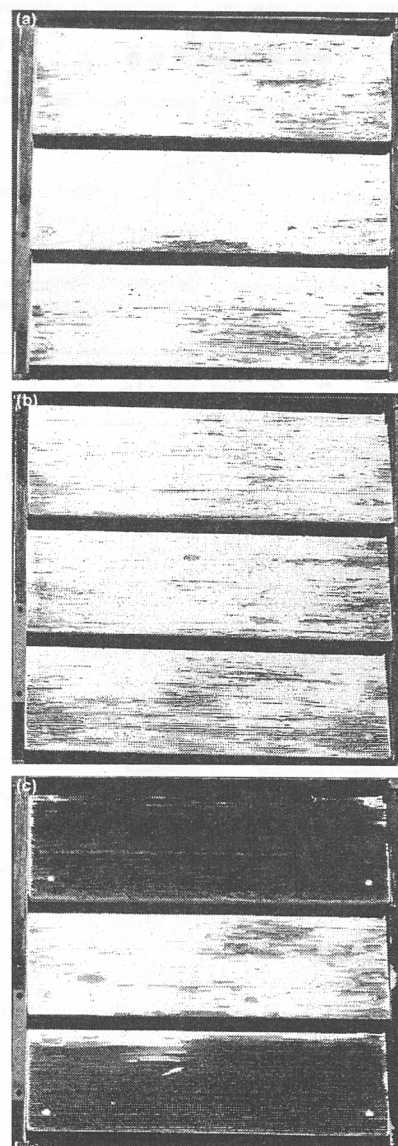
Figure 12. ~ Example of panels painted with one coat of latex primer and one coat of acrylic latex topcoat (latex/latex) after 20 years of outdoor exposure. (a) Control, no exposure prior to painting, (b) preweathered 1 week, and (c) preweathered 16 weeks.
