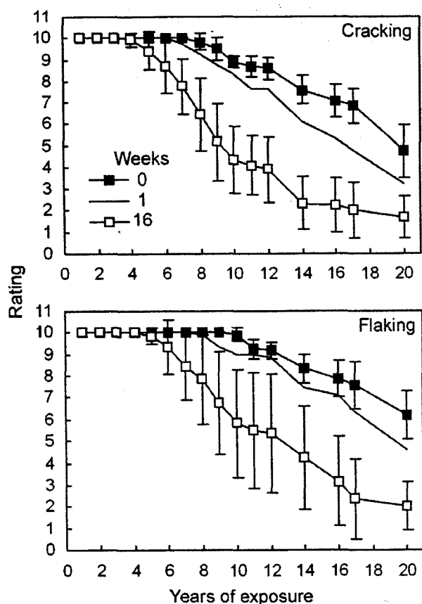
Figure 11. ~ Paint evaluations for cracking and flaking during 20 years of outdoor exposure for specimens finished with one coat of latex primer and one coat of acrylic latex topcoat (latex/latex). Data points are the average of 12 observations; bars show standard deviation.
