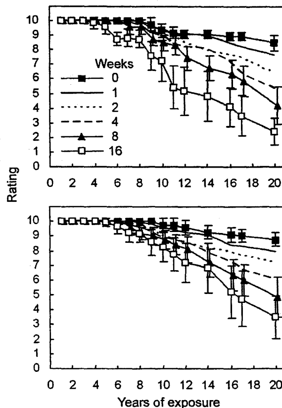
Figure 6. ~ Paint evaluations for cracking and flaking during 20 years for the paint system of solventborne water-repellent preservative, one coat of alkyd-oil primer, and one coat of acrylic latex topcoat (WRP/alkyd/latex). Data points are the average of 12 observations; bars show standard deviation.
