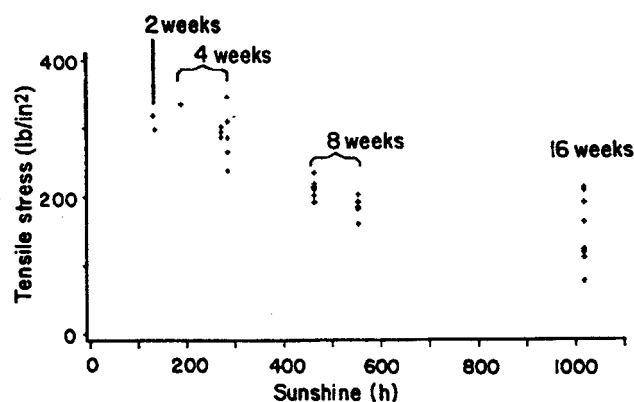
Figure 3. ~ Ultimate tensile stress compared with sunlight exposure time of acrylic latex primer on WRC. Only primerhood interphase failures are shown.
