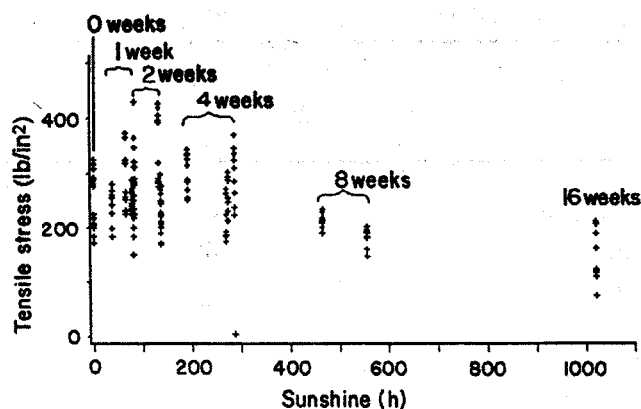
Figure 2. ~ Ultimate tensile stress compared with sunlight exposure time of acrylic latex primer on WRC. All adhesive failures and cohesive wood failures are shown.
