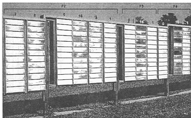
Figure 7. ~ Exposure fence west of Madison, Wisconsin, showing painted specimens after 20 years of outdoor exposure (F2, WRP/alkyd/latex; F3, alkyd/latex; F4, latex/latex; numbers are weeks of preweathering).
