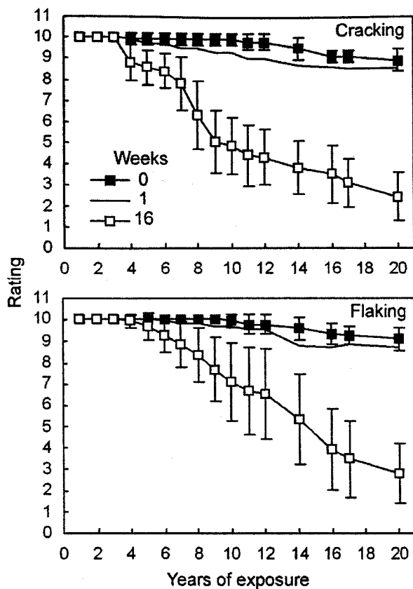
Figure 9. ~ Paint evaluations for cracking and flaking during 20 years of outdoor exposure for specimens painted with one coat of alkyd-oil primer and one coat of acrylic latex topcoat (alkyd/latex). Data points are the average of 12 observations; bars show standard deviation.
