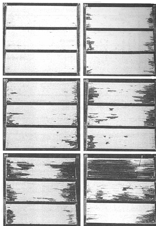
Figure 8. ~ Examples of panels painted with a solvent-borne water-repellent preservative, one coat of alkyd-oil primer, and one coat of acrylic latex topcoat (WRP/alkyd/latex) after 20 years of outdoor exposure. (a) Control, no exposure prior to painting, (b) preweathered 1 week, (c) preweathered 2 weeks, (d) preweathered 4 weeks, (e) preweathered 8 weeks, and (f) preweathered 16 weeks.
