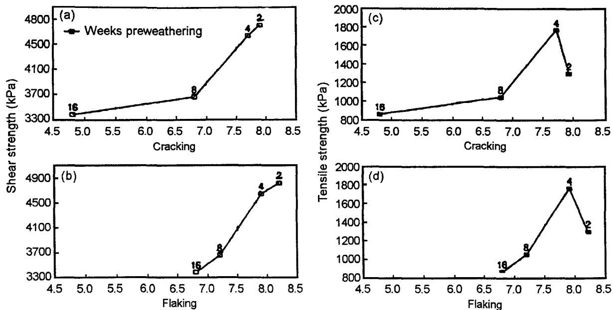
Figure 13. ~ Paint adhesive strength (shear and tension) of the alkyd-oil primer compared with the cracking or flaking evaluations of the WRP/alkyd/latex paint system after 17 years of outdoor exposure. (a) Shear strength vs. cracking, (b) shear strength vs. flaking, (c) tensile strength vs. cracking, and (d) tensile strength vs. flaking. Number of weeks of preweathering is shown with each data point. The r^2 values are 0.81, 0.98, 0.61, and 0.56 for (a) through (d), respectively. If the 2-week data are not included in the regression analysis for (c) and (d), the r^2 values are 0.73 and 0.97, respectively.
