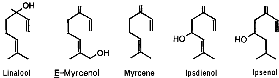
FIG. 1. Myrcene and its principal oxidation products.
