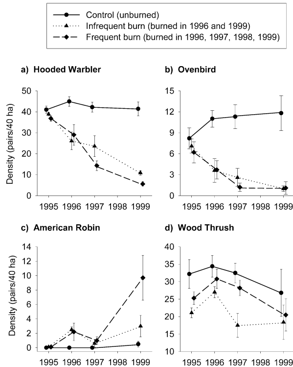
FIGURE 3. Mean (standard error) densities of bird species in relation to prescribed burning treatments in mixed-oak forests, southern Ohio; 1995 represents pre-burn conditions (Artman et al. 2001).
