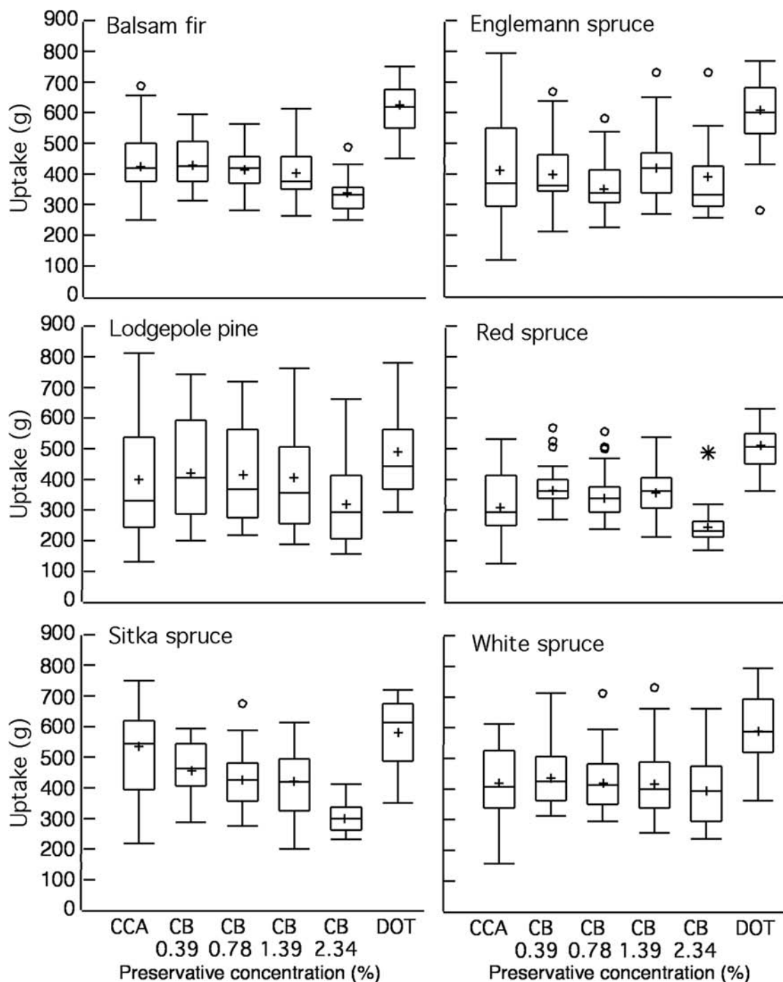
FIG. 2. Uptake (weight gain) for each preservative solution–wood species combination. Boxes depict data between 25th (Q1) and 75th (Q3) percentiles and represent interquartile range (IQR). Horizontal line across box indicates median; plus sign indicates mean. Lower whisker extending from bottom of box indicates data represented by Q1 - (1.5IQR) ; higher whisker extending from top of box is represented by Q3 + (1.5IQR) . Any data beyond these limits are plotted by a circle unless it exceeds either Q1 - (3IQR) or Q3 + (3.0IQR) . In this case, data are plotted by an asterisk.
