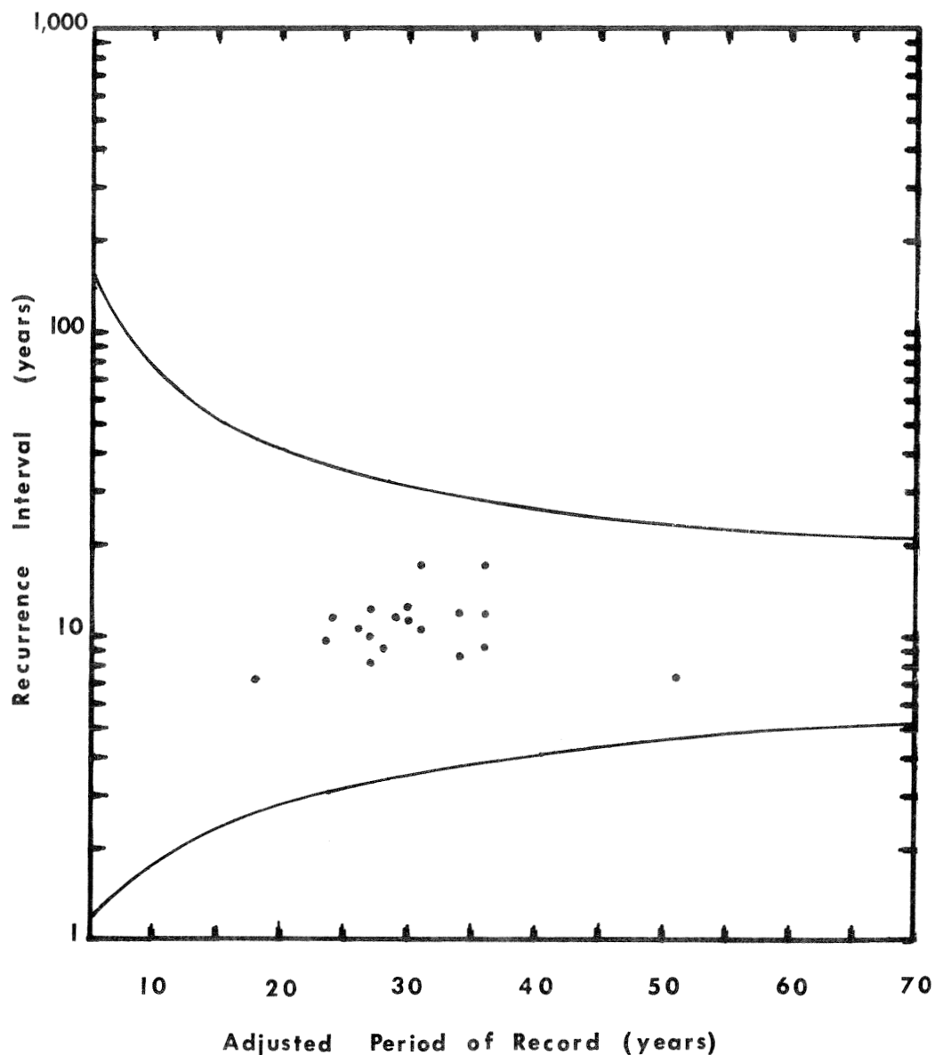
Figure 2.--Homogeneity of data for discharges at recurrence intervals of 10 years from both large and small watersheds. (The upper and lower lines are the 95-percent confidence limits.)
