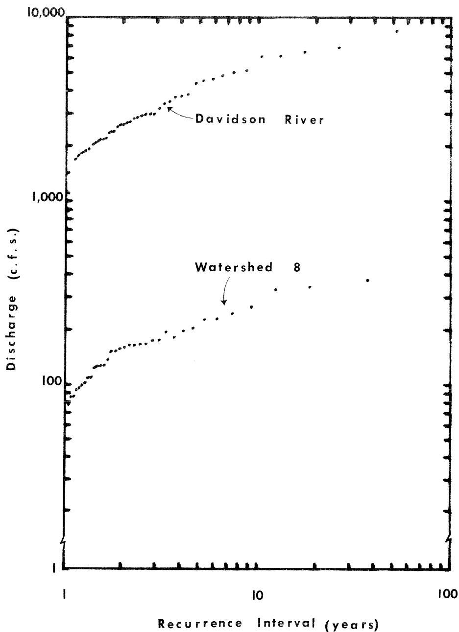
Figure 1.--Discharge vs. recurrence interval for Coweeta Watershed 8 (2.9 sq. mi.) and the Davidson River drainage (40 sq. mi.).
