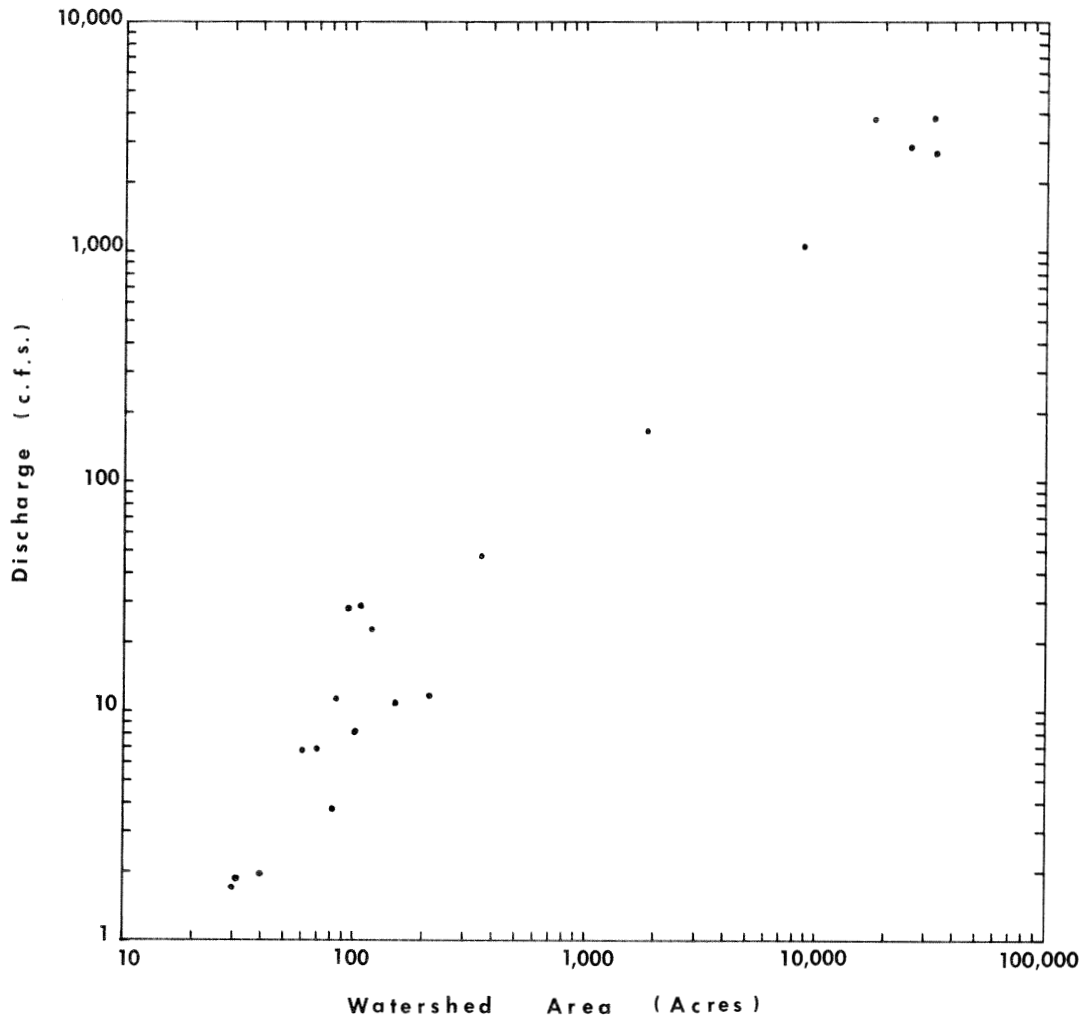
Figure 3.--Relationship between the mean annual discharge (2.33-year recurrence interval) and watershed area for both large and small watersheds.
