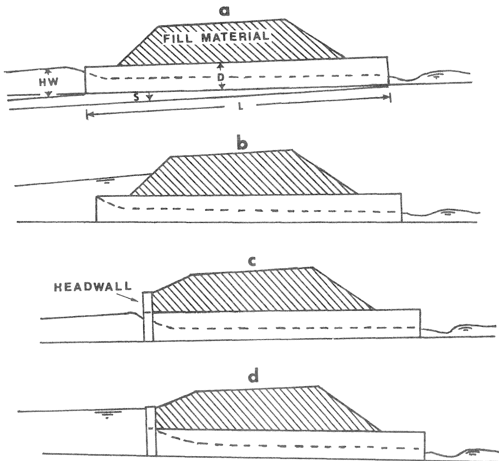
Figure 6.--Inlet control for two types of culverts and two depths of headwater. Schematics a and b illustrate culverts which project into the inlet basin. In a , headwater depth (HW) is equal to the culvert diameter (D) or rise of pipe-arch culverts; in b , headwater depth is greater than culvert diameter. The two examples of headwater depth are shown for culverts with headwalls in c and d . Other dimensions are culvert length (L) and slope (S).
