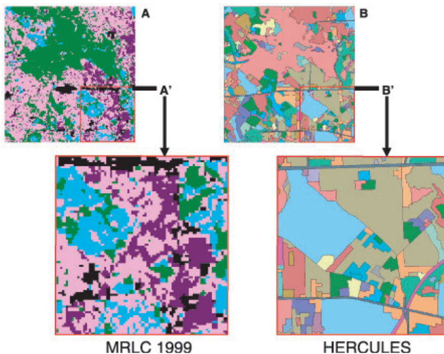
Fig. 3. Comparison of A) MultiResolution Land Cover (MRLC) and B) HERCULES land cover classifications for the Rognel Heights area of Baltimore in 1999. The southeast corner of each classification is enlarged in the lower panels (A' and B' respectively). MRLC shows forest, low, medium and high intensity residential, and commercial land covers. HERCULES differentiates between structurally dominated patches, vegetationally dominated patches, and patches that have different amounts of impervious surfaces.
