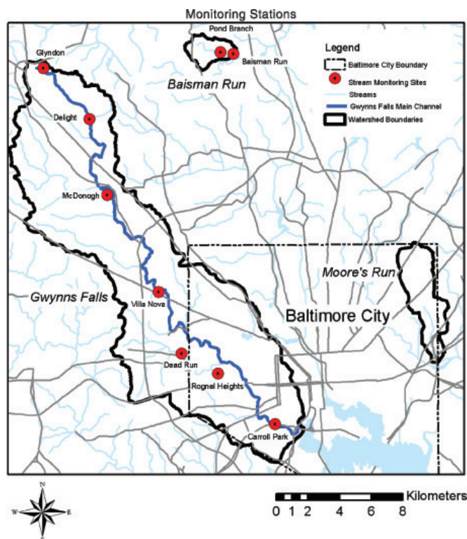
Fig. 2. Key watershed based sampling areas of the Baltimore Ecosystem Study LTER. Baisman Run contains the forested reference catchment of Ponds Branch, and a low density suburban catchment. The Gwynns Falls catchment samples suburban headwaters, residential and agricultural lands in middle reaches, and old residential, commercial, and industrial coverages in the lower reaches. Subwatershed sampling stations represent these different coverages, while the mainstem sampling stations at Carroll Park, Villa Nova, Delight, and Glyndon sample cumulative changes in water flow and quality.
