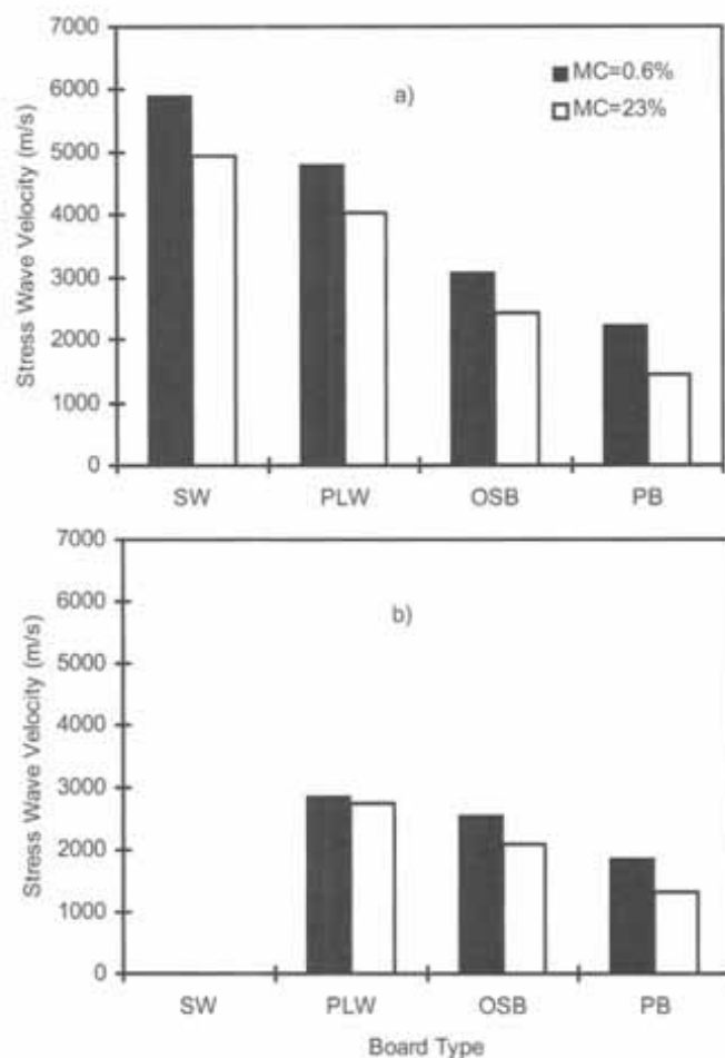
Figure 6. — A comparison of stress-wave velocity in solid wood (southern pine), plywood, OSB, and particleboard: a) parallel direction; and b) perpendicular direction. SW = solid wood; PLW = plywood; PB = particleboard.
