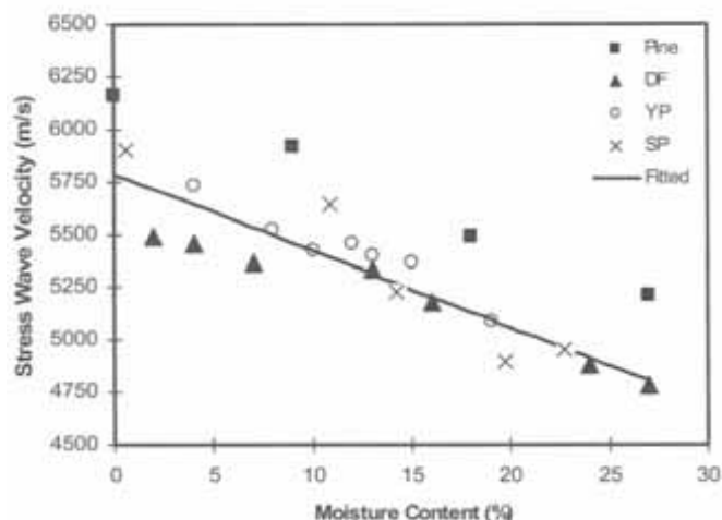
Figure 4. — A comparison of stress-wave velocity as a function of MC for several solid wood species along the longitudinal direction. DF = Douglas-fir; YP = yellow-poplar; SP = southern pine.
