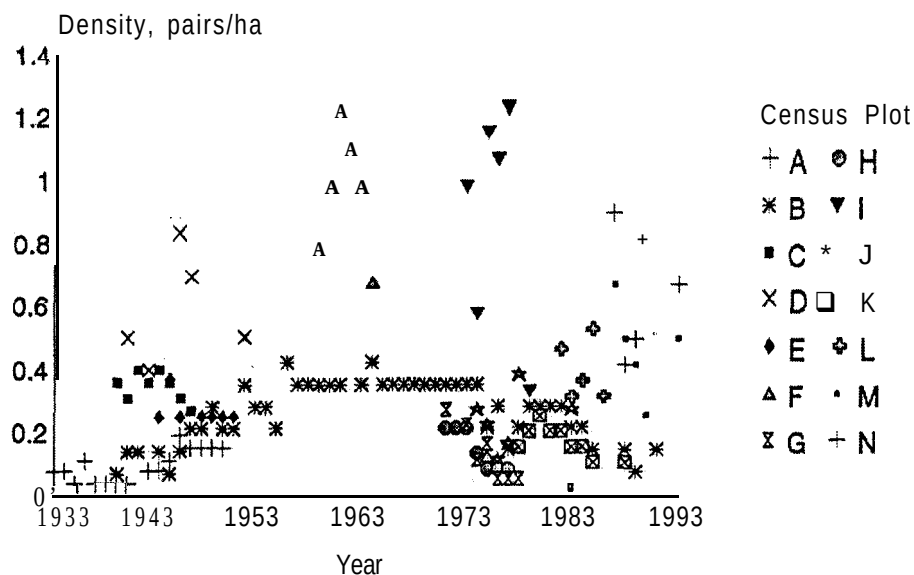
Figure3. Cerulean warbler breeding density as recorded on Breeding Bird Census plots. Only plots censused at least 5 times between 1932 and 1993 are included. Plots designated in figure, (Site reference number from Breeding Bird Census files), State, mean \pm standard deviation of density in pairs/ha (1 pr/ha = 0.4 pr/acre), sample size of years recorded, early and late years recorded on plot, are as follows: A (32001), OH, 0.10 \pm 0.05 , N=16, 1932-I 950; B (37200), OH, 0.26 \pm 0.10 , N=47, 1940-I 991; C (40030), OH, 0.35 \pm 0.05 , N=8, 1940-I 947; D (41037), OH, 0.58 \pm 0.18 , N=5, 1941-I 952; E (44027), VA, 0.26 \pm 0.05 , N=7, 1944-I 951; F (59010), IN, 0.84 \pm 0.36 , N=7, 1959-1975; G (71035), MD, 0.13 \pm 0.09 , N=7, 1971-1978; H (71036), MD, 0.14 \pm 0.06 , N=7, 1971-1977; I (73092), OH, 0.89 \pm 0.36 , N=6, 1973-I 979; J (74131), PA, 0.24 \pm 0.10 , N=6, 1974-I 983; K (78237), OH, 0.16 \pm 0.05 , N=9, 1978-I 987; L (82314), PA, 0.39 \pm 0.09 , N=5, 1982-I 986; M (83031), VA, 0.38 \pm 0.22 , N=6, 1983-I 993; N (87013), VA, 0.66 \pm 0.21 , N=5, 1987-1993.
