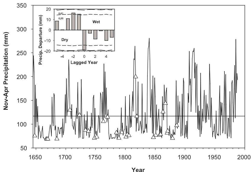
Figure 4 —November to April precipitation (1650 to 1989) and the 30 most synchronous fire years among the Sky Islands (labeled dates from 1650 to 1900 in figure 3). The inset graph in upper left corner shows the results of the superposed epoch analysis, with average conditions significantly dry ( p < 0.01 ) during the 30 synchronous fire years, and the previous two years significantly wet ( p < 0.05 ) (see text for explanation).
