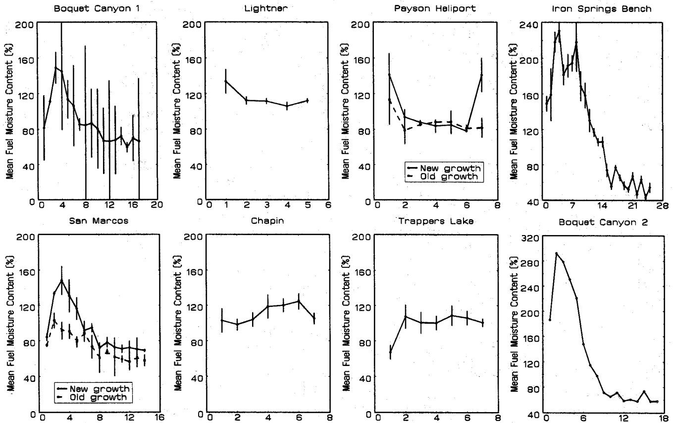
Figure 1. Mean live moisture content of shrub and canopy fuels sampled at locations in southern California, Arizona, and Colorado during one growing season. Vertical lines indicated 95% confidence intervals. The X-axis is sample time (1 denoting 1st sample collection, 2 denoting 2nd sample collection, etc.). Chamise was sampled at Boquet Canyon 1 and San Marcos, Gambel oak at Lightner, turbinella oak at Payson Heliport, sagebrush at Iron Springs Bench, pinon at Chapin, Engelmann spruce at Trappers Lake, and black sage at Boquet Canyon 2.
