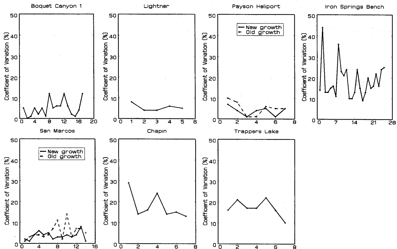
Figure 2. Coefficient of variation of live moisture content of shrub and canopy fuel samples collected at locations in southern California, Arizona, and Colorado during one growing season. The X-axis is sample time (1 denoting 1st sample collection, 2 denoting 2nd sample collection, etc.). Chamise was sampled at Boquet Canyon 1 and San Marcos, Gambel oak at Lightner, turbinella oak at Payson Heliport, sagebrush at Iron Springs Bench, pinon at Chapin, Engelmann spruce at Trappers Lake, and black sage at Boquet Canyon 2.
