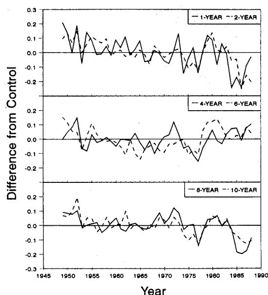
Figure 5. Difference in growth between fire rotation treatment trees and control trees calculated as the difference in their respective BAI index values. Positive values indicate growth less than that of control trees. Negative values indicate growth less than that of control trees.
