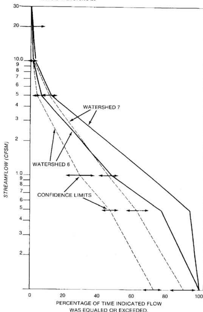
Figure 3.—Effects of deforestation on flow duration, hydrologic year 1969. Solid lines represent measured flow duration; dashed lines are estimated flow duration before deforestation, as derived from regression on measured flow duration from the forested watershed.
