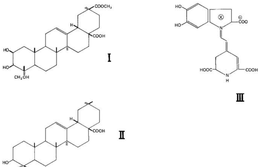
Figure 2.—Structures of (I) phytolaccagenin, (II) oleanic acid, and (III) betanin.
