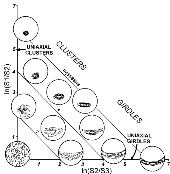
Fig. 5. Normalized eigenvalue ratios of directional data. The ratio \ln(S_1/S_2) predicts the degree of data clustering and \ln(S_2/S_3) describes the tendency of data to plot in a girdle pattern. The ratio \ln(S_1/S_3) expresses how strongly the orientation vectors are grouped without specifying any pattern of assemblage. Modified from Woodcock (1977).
