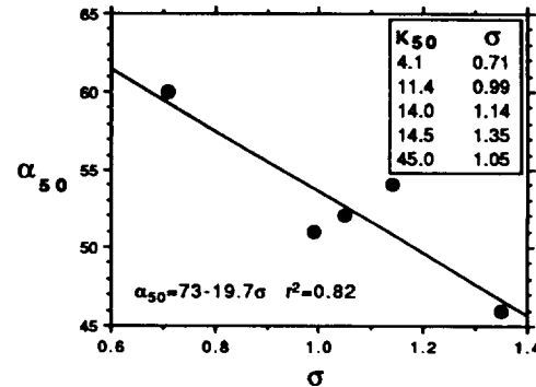
Fig. 8. Correlation of sorting, \sigma , and \alpha_{50} for the five samples. Sorting parameters calculated according to the method presented by Blatt et al. [1980] (see notes for Table 2).
