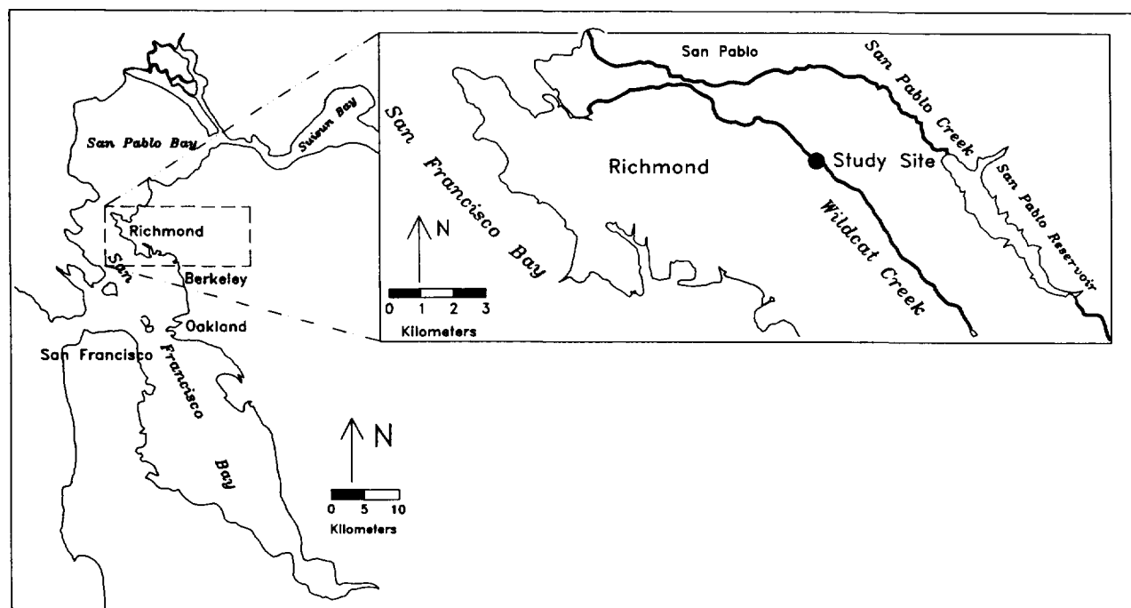
Fig. 1. Study site location map within the bay area of northern California.
