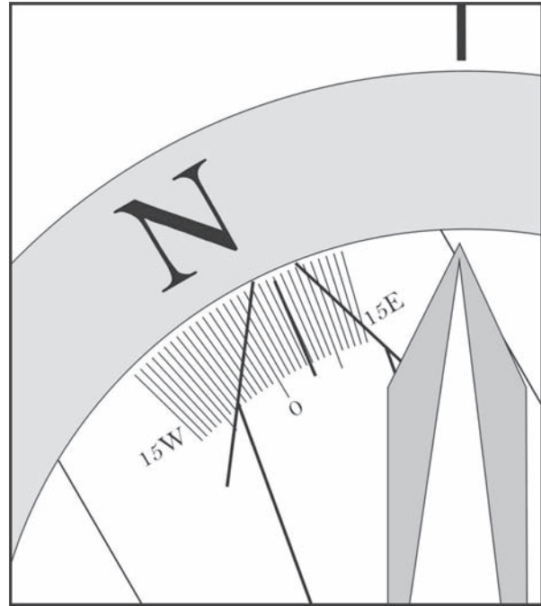
Figure HT-15 —The mark in the orienting arrow indicates the compass is set to 6 degrees east declination.
