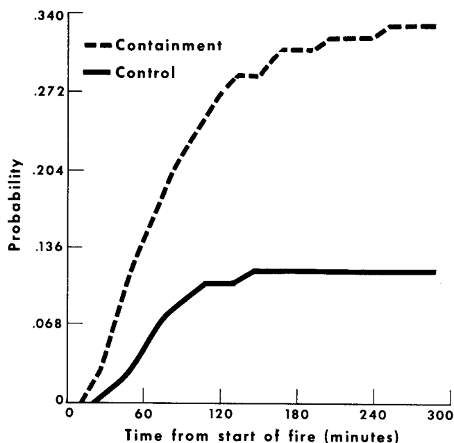
Figure 8 —Sample computer output of the Initial Attack Assessment Model. Both predicted fire growth and probable success of the dispatched forces are shown.
