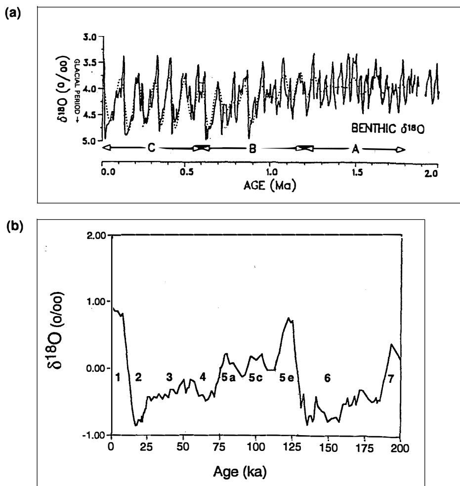
FIG. 2--(a) Benthic oxygen isotope curve ( \delta^{18}\text{O} ) from the Atlantic Ocean for the past 2 million years showing the lower intensity, shorter cycle (41-kyr) fluctuations of the first million years of the Quaternary and the 100-kyr cycle of the last million years (modified from Imbrie et al. 1992); (b) Oxygen isotope curve for the last 200,000 years showing standard oxygen-isotope stages (OIS). Odd-numbered OIS stages are interglacials or interstadials, even numbered stages are glacial or pluvial stages.
