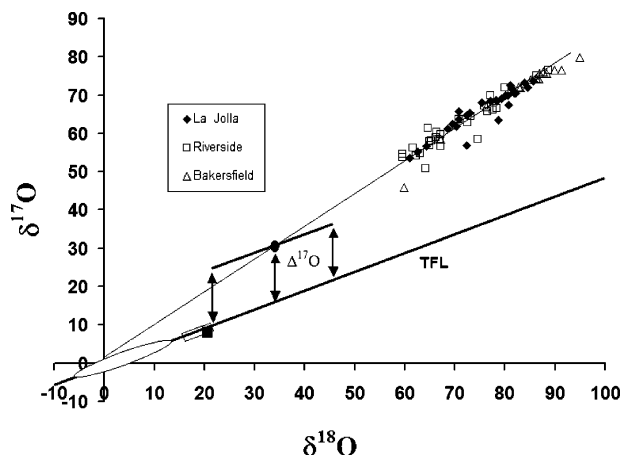
FIGURE 2. Oxygen three isotope plot of \text{NO}_3^- -atm from the Riverside Air Basin ( \square ), La Jolla, CA ( \blacklozenge ), and Bakersfield, CA ( \triangle ), showing an average \Delta^{17}\text{O} of 25 \pm 4\text{‰} and a high correlation between \delta^{17}\text{O} and \delta^{18}\text{O} . The solid bold line is the terrestrial fractionation line (TFL) that describes most nonphotochemical isotopic compositions ( \delta^{17}\text{O} = 0.52(\delta^{18}\text{O}) ) including \text{NO}_3^- from nitrification (white oval), fertilizer \text{NO}_3^- (open rectangle), and air \text{O}_2 (solid square). Mixing between \text{NO}_3^- -atm and \text{NO}_3^- from nitrification or fertilizer decreases the \Delta^{17}\text{O} proportionally to the respective source strengths (solid circle). Once mixed, any subsequent kinetic or equilibrium isotopic fractionations (denitrification/reduction) follow \delta^{17}\text{O} = 0.52(\delta^{18}\text{O}) , i.e., parallel to the terrestrial fractionation line, leaving the \Delta^{17}\text{O} unaltered (arrows). Our overall \text{NO}_3^- -atm \delta^{18}\text{O} values are larger (60–95‰) than those of other studies (40–75‰) but with similar spreads (35‰) and are likely due to recent evidence showing offline \text{NO}_3^- \delta^{18}\text{O} experimental methods suffer from scaling factors for samples that differ significantly from \delta^{18}\text{O} near 23‰ (30).
