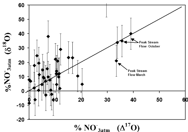
FIGURE 4. Mass balance estimates of the percentage of \text{NO}_3^-_{\text{atm}} in terrestrial \text{NO}_3^- samples using an average \text{NO}_3^-_{\text{atm}} \delta^{18}\text{O} = 70\text{‰} and \Delta^{17}\text{O} = 25\text{‰} and a nitrification \text{NO}_3^- \delta^{18}\text{O} of 3\text{‰} , \Delta^{17}\text{O} = -0.1 . The solid line is a 1:1 correlation slope if the \delta^{18}\text{O} method and the \Delta^{17}\text{O} method gave the same percentage of \text{NO}_3^-_{\text{atm}} . Error bars represent uncertainties using solely the \delta^{18}\text{O} values due to the range of possible nitrification \delta^{18}\text{O} values from -5\text{‰} to +15\text{‰} . Zero or negative percent would be interpreted as having no \text{NO}_3^-_{\text{atm}} . Peak streamflow during the October storm results in good agreement between \delta^{18}\text{O} and \Delta^{17}\text{O} methods. No correlation exists in later storms (March), and there is little agreement during base streamflow conditions or for soil \text{NO}_3^- .
