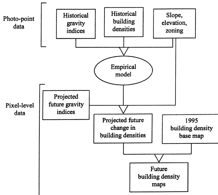
Figure 2. General modeling procedure.
