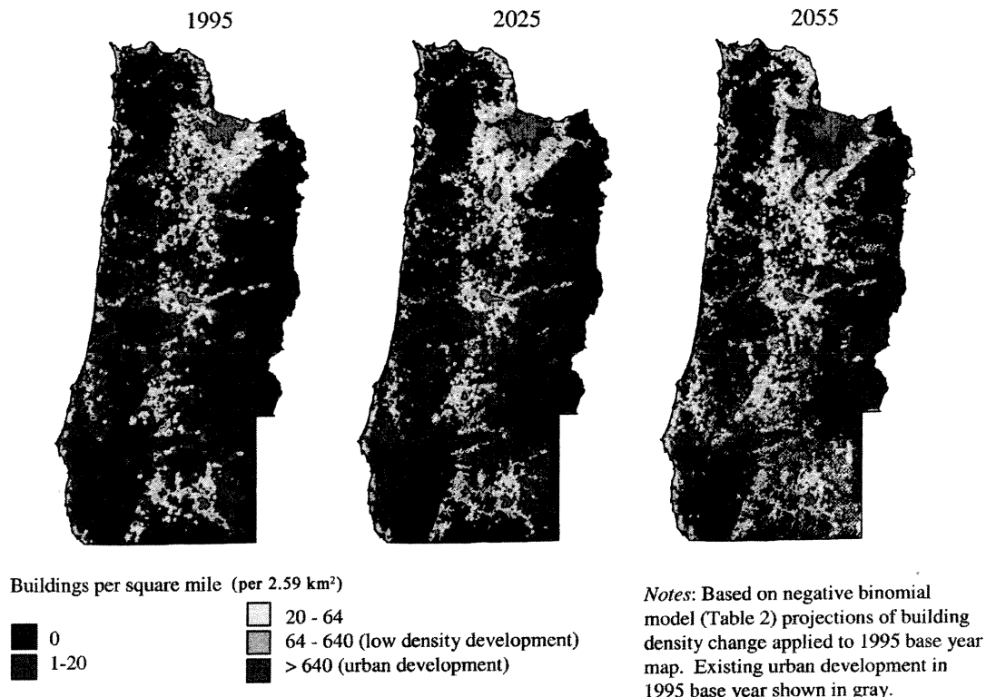
Figure 3. Projected building density classes in Western Oregon.
