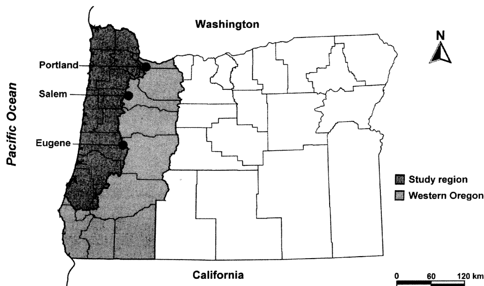
Figure 1. Coastal landscape analysis and modeling study region in Western Oregon.
