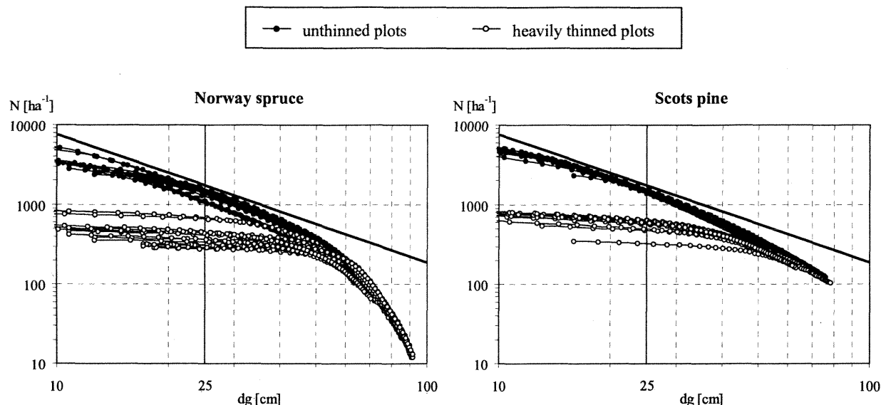
Figure 2. Relationship between stem number per hectare ( N ) and quadratic mean diameter ( d_g ) on the log-log scale for stands of Norway spruce ( Picea abies L. Karst.) and Scots pine ( Pinus sylvestris L.). Stand development has been simulated for 250 years using the forest stand growth model PROGNAUS. The bold lines follow the slope of -1.605 postulated by Reineke (1933). On heavily thinned plots 85% of the trees were removed randomly before the simulation runs had been started. Plots with moderate thinning are not displayed in this graph.
