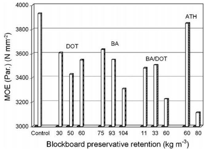
Fig. 5 Parallel-to-plane MOE as function of retardant retention in blockboards
